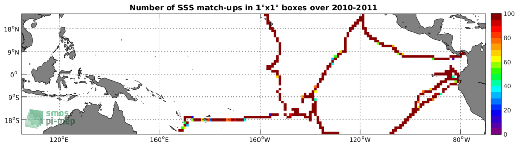
Figure 4: Number of SSS match-ups between TSG-GOSUD-Sailing-ship SSS and the SMOS-L3-BEC-OA-V1-9DAYS-0.25DEG SSS product for the Tropical Pacific Ocean Pi-MEP region over 1^\circ \times 1^\circ boxes and for the full satellite product period.
