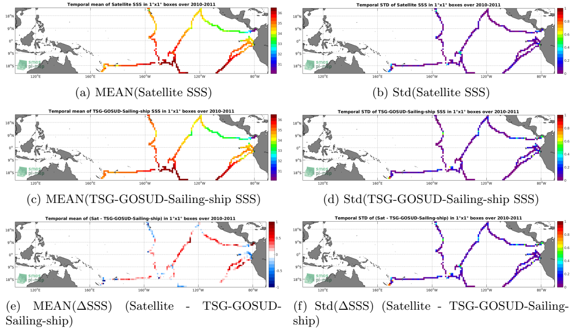
Figure 6: Temporal mean (left) and Std (right) of SSS from SMOS-L3-BEC-OA-V1-9DAYS-0.25DEG (top), TSG-GOSUD-Sailing-ship (middle), and of \Delta SSS (Satellite - TSG-GOSUD-Sailing-ship). Only match-up pairs are used to generate these maps.
