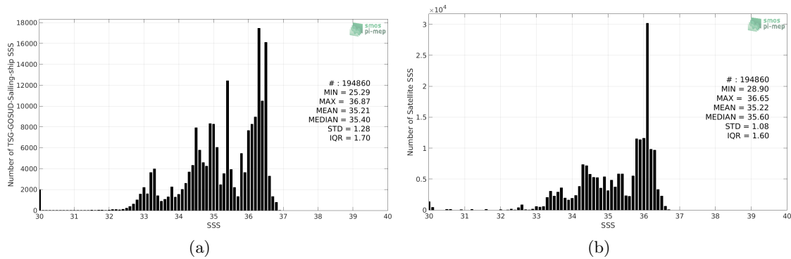
Figure 2: Histograms of SSS from TSG-GOSUD-Sailing-ship (a) and SMOS-L3-BEC-OA-V1-9DAYS-0.25DEG (b) considering all match-up pairs per bins of 0.1 over the Tropical Pacific Ocean Pi-MEP region and for the full satellite product period.
