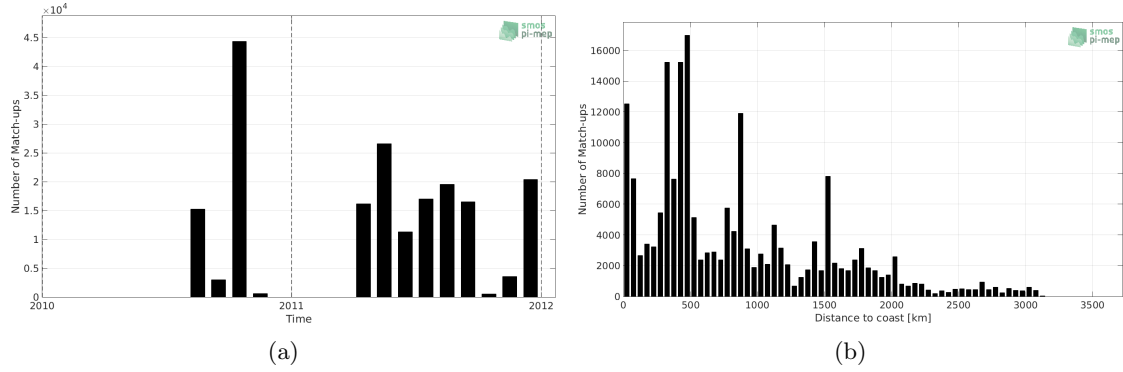
Figure 1: Number of match-ups between TSG-GOSUD-Sailing-ship and SMOS-L3-BEC-OA-V1-9DAYS-0.25DEG SSS as a function of time (a) and as function of the distance to coast (b) over the Tropical Pacific Ocean Pi-MEP region and for the full satellite product period.
