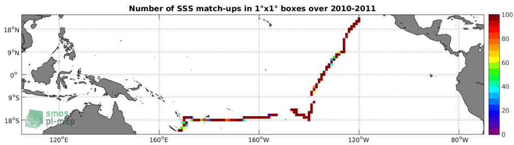
Figure 4: Number of SSS match-ups between TSG-GOSUD-Sailing-ship SSS and the SMOS-L3-BEC-OA-V1-9DAYS-0.25DEG SSS product for the Tropical Pacific Ocean Pi-MEP region over 1^{\circ} \times 1^{\circ} boxes and for the full satellite product period.
