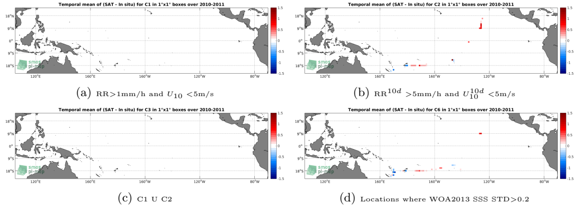
Figure 12: Temporal mean gridded over spatial boxes of size 1^\circ \times 1^\circ of \Delta SSS (SMOS-L3-BEC-OA-V1-9DAYS-0.25DEG - TSG-GOSUD-Sailing-ship) for 4 different subdatasets corresponding to: RR > 1\text{mm/h} and U_{10} < 5\text{m/s} (a), RR^{10d} > 5\text{mm/h} and U_{10}^{10d} < 5\text{m/s} (b), C1 U C2 (c), Locations where WOA2013 SSS STD > 0.2 (d).
