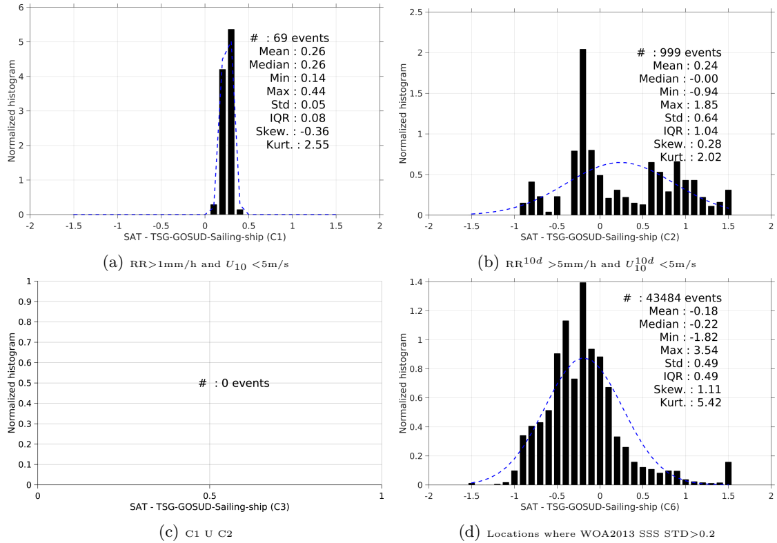
Figure 13: Normalized histogram of \Delta SSS (SMOS-L3-BEC-OA-V1-9DAYS-0.25DEG - TSG-GOSUD-Sailing-ship) for 6 different subdatasets corresponding to: RR > 1mm/h and U_{10} < 5 m/s (a), RR^{10d} > 5 mm/h and U_{10}^{10d} < 5 m/s (b), C1 U C2 (c), Locations where WOA2013 SSS STD > 0.2 (d).
