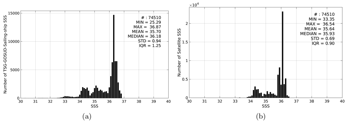
Figure 2: Histograms of SSS from TSG-GOSUD-Sailing-ship (a) and SMOS-L3-BEC-OA-V1-9DAYS-0.25DEG (b) considering all match-up pairs per bins of 0.1 over the Tropical Pacific Ocean Pi-MEP region and for the full satellite product period.
