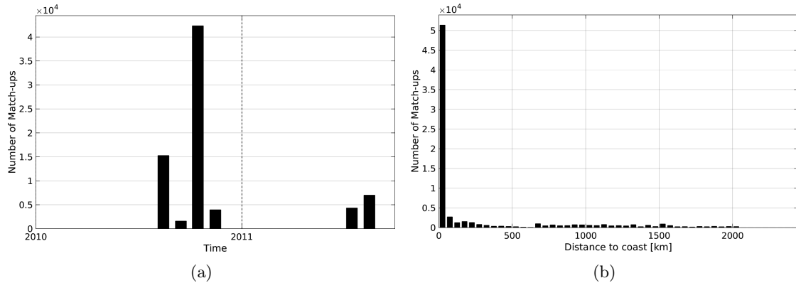
Figure 1: Number of match-ups between TSG-GOSUD-Sailing-ship and SMOS-L3-BEC-OA-V1-9DAYS-0.25DEG SSS as a function of time (a) and as function of the distance to coast (b) over the Tropical Pacific Ocean Pi-MEP region and for the full satellite product period.
