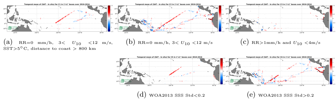
Figure 12: Temporal mean gridded over spatial boxes of size 1^\circ \times 1^\circ of \Delta SSS (SMOS-L3-BEC-OA-V1-9DAYS-0.25DEG - TSG-GOSUD-Research-vessel) for 5 different subdatasets corresponding to: RR=0 mm/h, 3 < U_{10} < 12 m/s, SST > 5^\circ\text{C} , distance to coast > 800 km (a), RR=0 mm/h, 3 < U_{10} < 12 m/s (b), RR > 1 mm/h and U_{10} < 4 m/s (c), WOA2013 SSS Std < 0.2 (d), WOA2013 SSS Std > 0.2 (e).
