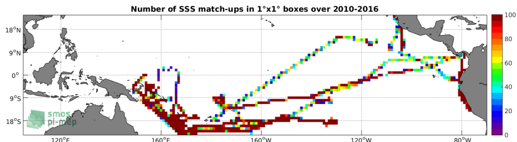
Figure 4: Number of SSS match-ups between TSG-GOSUD-Research-vessel SSS and the SMOS-L3-BEC-OA-V1-9DAYS-0.25DEG SSS product for the Tropical Pacific Ocean Pi-MEP region over 1^\circ \times 1^\circ boxes and for the full satellite product period.
