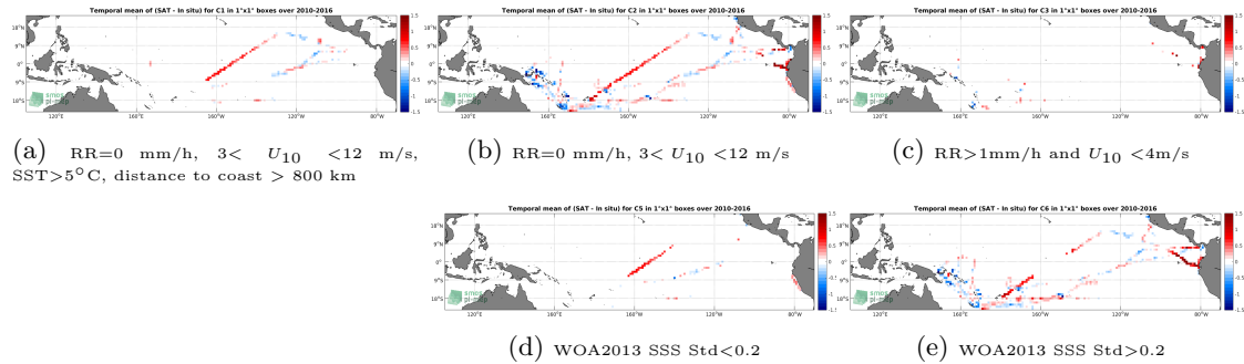
Figure 12: Temporal mean gridded over spatial boxes of size 1^\circ \times 1^\circ of \Delta SSS (SMOS-L3-BEC-OA-V1-9DAYS-0.25DEG - TSG-GOSUD-Research-vessel) for 5 different subdatasets corresponding to:RR=0 mm/h, 3 < U_{10} < 12 m/s, SST >5^\circ C, distance to coast > 800 km (a), RR=0 mm/h, 3 < U_{10} < 12 m/s (b), RR >1 mm/h and U_{10} < 4 m/s (c), WOA2013 SSS Std <0.2 (d), WOA2013 SSS Std >0.2 (e).
