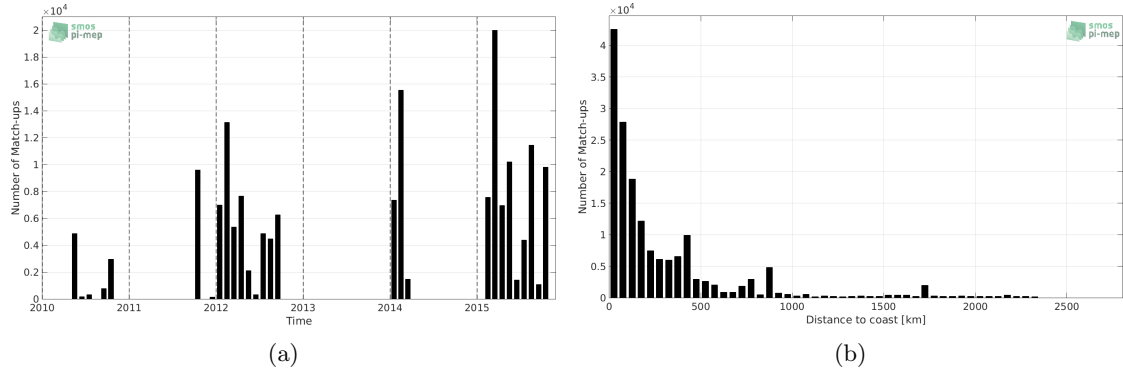
Figure 1: Number of match-ups between TSG-GOSUD-Research-vessel and SMOS-L3-BEC-OA-V1-9DAYS-0.25DEG SSS as a function of time (a) and as function of the distance to coast (b) over the Tropical Pacific Ocean Pi-MEP region and for the full satellite product period.
