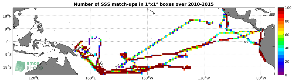
Figure 4: Number of SSS match-ups between TSG-GOSUD-Research-vessel SSS and the SMOS-L3-BEC-OA-V1-9DAYS-0.25DEG SSS product for the Tropical Pacific Ocean Pi-MEP region over 1^\circ \times 1^\circ boxes and for the full satellite product period.
