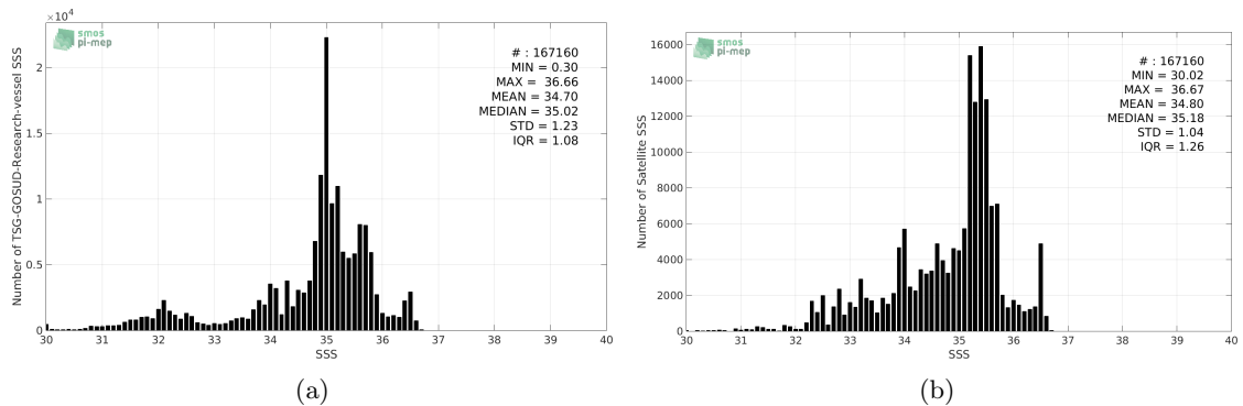
Figure 2: Histograms of SSS from TSG-GOSUD-Research-vessel (a) and SMOS-L3-BEC-OA-V1-9DAYS-0.25DEG (b) considering all match-up pairs per bins of 0.1 over the Tropical Pacific Ocean Pi-MEP region and for the full satellite product period.
