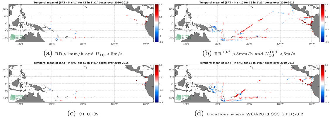
Figure 12: Temporal mean gridded over spatial boxes of size 1^\circ \times 1^\circ of \Delta SSS (SMOS-L3-BEC-OA-V1-9DAYS-0.25DEG - TSG-GOSUD-Research-vessel) for 4 different subdatasets corresponding to: RR > 1\text{mm/h} and U_{10} < 5\text{m/s} (a), RR^{10d} > 5\text{mm/h} and U_{10}^{10d} < 5\text{m/s} (b), C1 U C2 (c), Locations where WOA2013 SSS STD > 0.2 (d).
