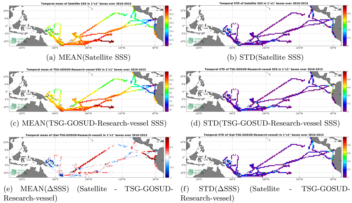
Figure 6: Temporal mean (left) and STD (right) of SSS from SMOS-L3-BEC-OA-V1-9DAYS-0.25DEG (top), TSG-GOSUD-Research-vessel (middle), and of \Delta SSS (Satellite - TSG-GOSUD-Research-vessel). Only match-up pairs are used to generate these maps.
