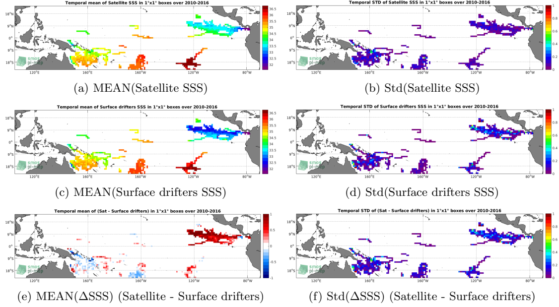
Figure 5: Temporal mean (left) and Std (right) of SSS from SMOS-L3-BEC-OA-V1-9DAYS-0.25DEG (top), Surface drifters (middle), and of \Delta SSS (Satellite - Surface drifters). Only match-up pairs are used to generate these maps.
