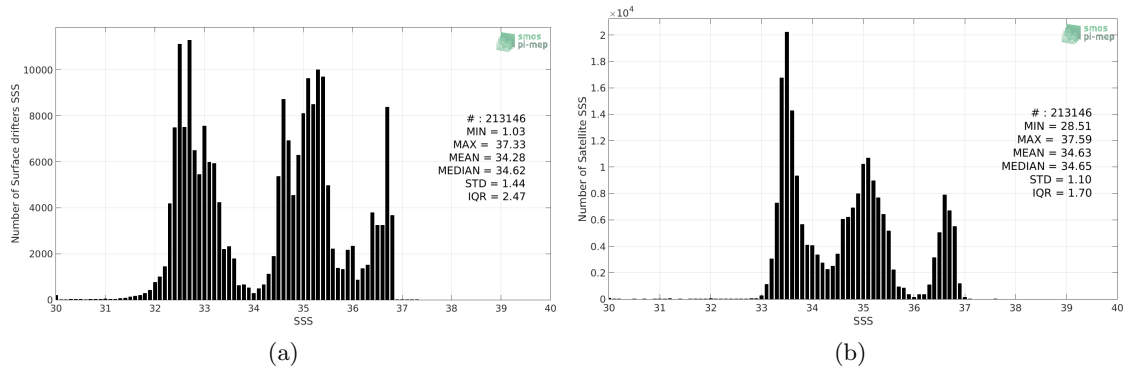
Figure 2: Histograms of SSS from Surface drifters (a) and SMOS-L3-BEC-OA-V1-9DAYS-0.25DEG (b) considering all match-up pairs per bins of 0.1 over the Tropical Pacific Ocean Pi-MEP region and for the full satellite product period.
