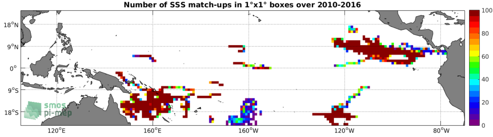
Figure 3: Number of SSS match-ups between Surface drifters SSS and the SMOS-L3-BEC-OA-V1-9DAYS-0.25DEG SSS product for the Tropical Pacific Ocean Pi-MEP region over 1^\circ \times 1^\circ boxes and for the full satellite product period.
