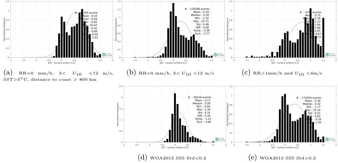
Figure 12: Normalized histogram of \Delta SSS (SMOS-L3-BEC-OA-V1-9DAYS-0.25DEG - Surface drifters) for 5 different subdatasets corresponding to: RR=0 mm/h, 3 < U_{10} < 12 m/s, SST > 5°C, distance to coast > 800 km (a), RR=0 mm/h, 3 < U_{10} < 12 m/s (b), RR > 1mm/h and U_{10} < 4 m/s (c), WOA2013 SSS Std < 0.2 (d), WOA2013 SSS Std > 0.2 (e).
