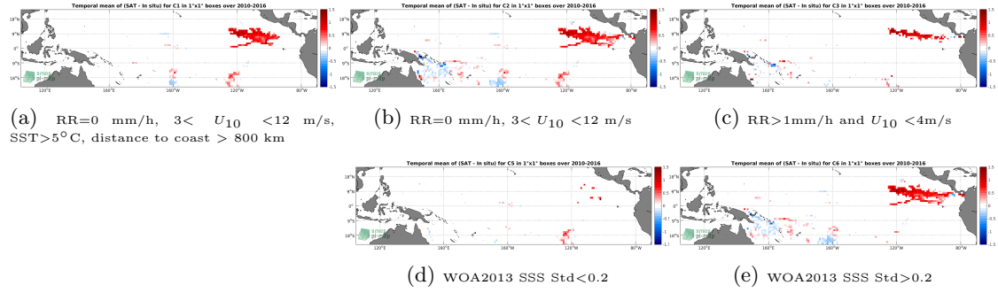
Figure 11: Temporal mean gridded over spatial boxes of size 1^\circ \times 1^\circ of \Delta SSS (SMOS-L3-BEC-OA-V1-9DAYS-0.25DEG - Surface drifters) for 5 different subdatasets corresponding to: RR=0 mm/h, 3 < U_{10} < 12 m/s, SST > 5^\circ C , distance to coast > 800 km (a), RR=0 mm/h, 3 < U_{10} < 12 m/s (b), RR > 1 mm/h and U_{10} < 4 m/s (c), WOA2013 SSS Std < 0.2 (d), WOA2013 SSS Std > 0.2 (e).
