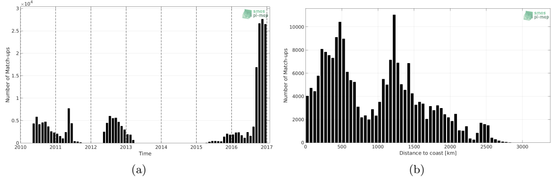
Figure 1: Number of match-ups between Surface drifters and SMOS-L3-BEC-OA-V1-9DAYS-0.25DEG SSS as a function of time (a) and as function of the distance to coast (b) over the Tropical Pacific Ocean Pi-MEP region and for the full satellite product period.
