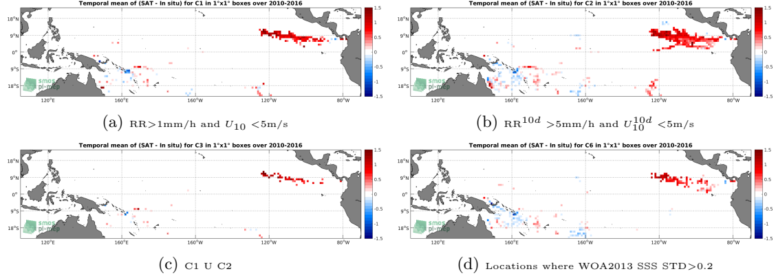
Figure 11: Temporal mean gridded over spatial boxes of size 1^\circ \times 1^\circ of \Delta SSS (SMOS-L3-BEC-OA-V1-9DAYS-0.25DEG - Surface drifters) for 4 different subdatasets corresponding to: RR > 1\text{mm/h} and U_{10} < 5\text{m/s} (a), RR^{10d} > 5\text{mm/h} and U_{10}^{10d} < 5\text{m/s} (b), C1 U C2 (c), Locations where WOA2013 SSS STD > 0.2 (d).
