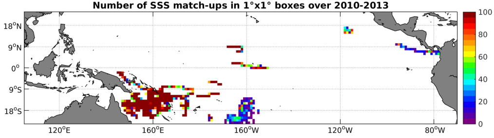
Figure 3: Number of SSS match-ups between Surface drifters SSS and the SMOS-L3-BEC-OA-V1-9DAYS-0.25DEG SSS product for the Tropical Pacific Ocean Pi-MEP region over 1^\circ \times 1^\circ boxes and for the full satellite product period.
