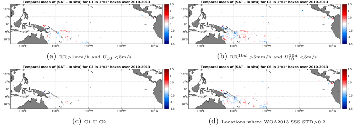
Figure 11: Temporal mean gridded over spatial boxes of size 1^\circ \times 1^\circ of \Delta SSS (SMOS-L3-BEC-OA-V1-9DAYS-0.25DEG - Surface drifters) for 4 different subdatasets corresponding to: RR > 1\text{mm/h} and U_{10} < 5\text{m/s} (a), RR^{10d} > 5\text{mm/h} and U_{10}^{10d} < 5\text{m/s} (b), C1 U C2 (c), Locations where WOA2013 SSS STD > 0.2 (d).
