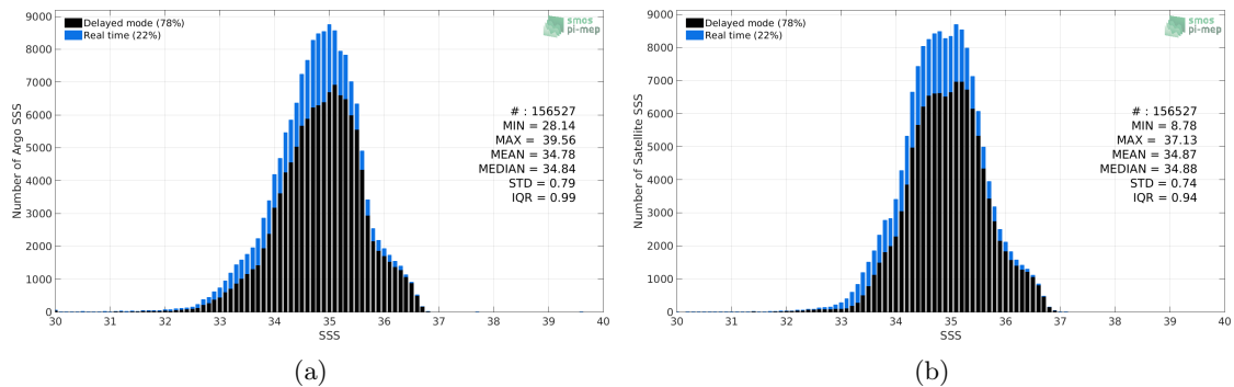
Figure 2: Histograms of SSS from Argo (a) and SMOS-L3-BEC-OA-V1-9DAYS-0.25DEG (b) considering all match-up pairs per bins of 0.1 over the Tropical Pacific Ocean Pi-MEP region and for the full satellite product period.
