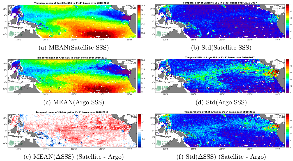
Figure 6: Temporal mean (left) and Std (right) of SSS from SMOS-L3-BEC-OA-V1-9DAYS-0.25DEG (top), Argo (middle), and of \Delta SSS (Satellite - Argo). Only match-up pairs are used to generate these maps.
