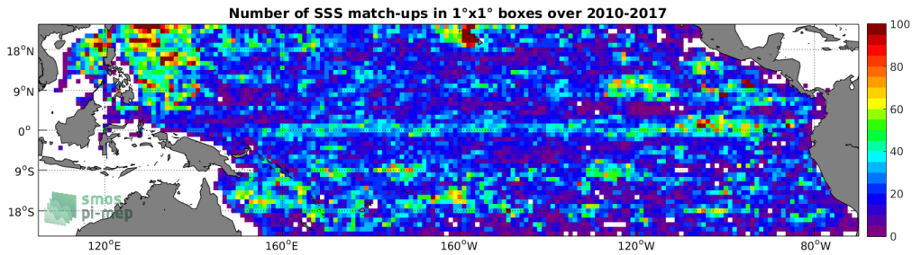
Figure 4: Number of SSS match-ups between Argo SSS and the SMOS-L3-BEC-OA-V1-9DAYS-0.25DEG SSS product for the Tropical Pacific Ocean Pi-MEP region over 1^\circ \times 1^\circ boxes and for the full satellite product period.
