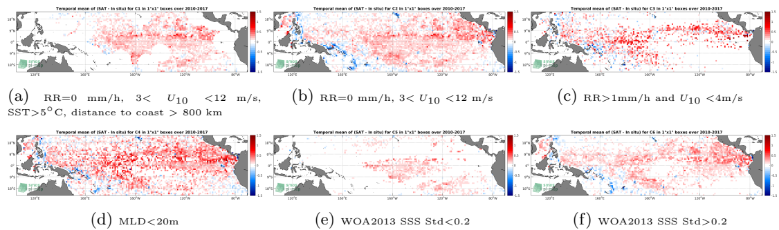
Figure 12: Temporal mean gridded over spatial boxes of size 1^\circ \times 1^\circ of \Delta SSS (SMOS-L3-BEC-OA-V1-9DAYS-0.25DEG - Argo) for 6 different subdatasets corresponding to:RR=0 mm/h, 3 < U_{10} < 12 m/s, SST >5^\circ C, distance to coast > 800 km (a), RR=0 mm/h, 3 < U_{10} < 12 m/s (b), RR >1 mm/h and U_{10} < 4 m/s (c),MLD <20 m (d),WOA2013 SSS Std <0.2 (e),WOA2013 SSS Std >0.2 (f).
