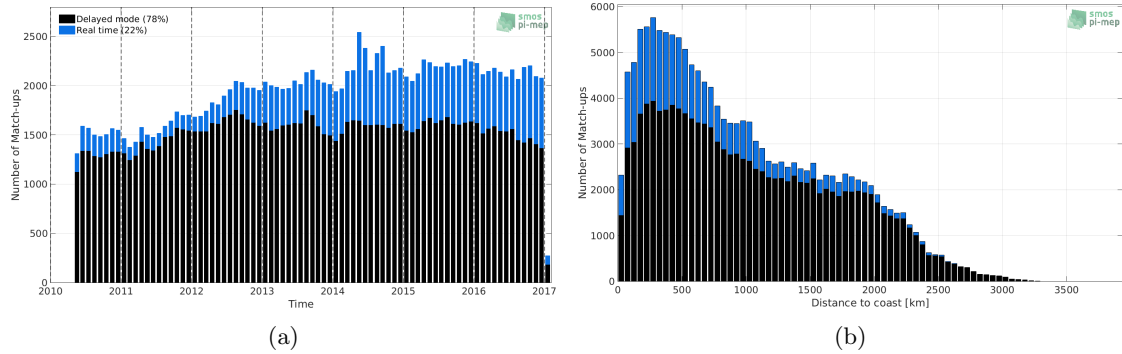
Figure 1: Number of match-ups between Argo and SMOS-L3-BEC-OA-V1-9DAYS-0.25DEG SSS as a function of time (a) and as function of the distance to coast (b) over the Tropical Pacific Ocean Pi-MEP region and for the full satellite product period.
