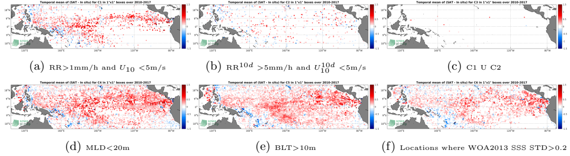
Figure 12: Temporal mean gridded over spatial boxes of size 1°x1° of \Delta SSS (SMOS-L3-BEC-OA-V1-9DAYS-0.25DEG - Argo) for 6 different subdatasets corresponding to:RR>1mm/h and U_{10} < 5m/s (a), RR^{10d} > 5mm/h and U_{10}^{10d} < 5m/s (b), C1 U C2 (c),MLD<20m (d),BLT>10m (e),Locations where WOA2013 SSS STD>0.2 (f).
