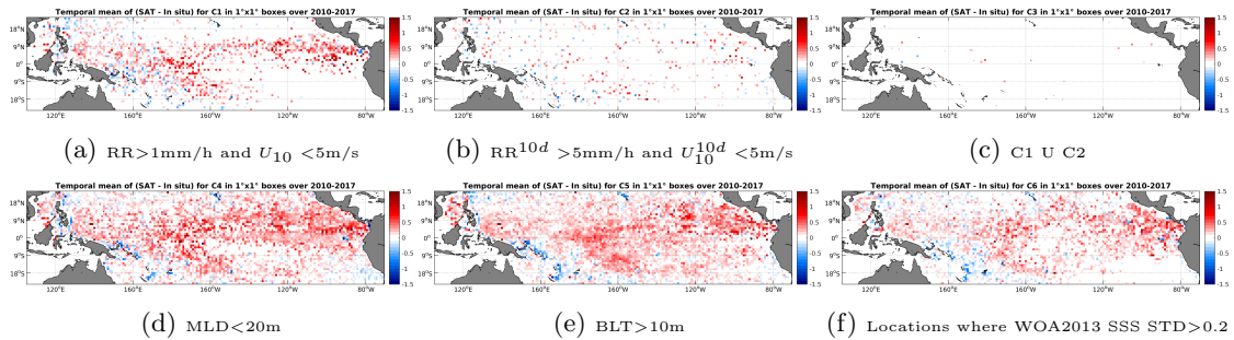
Figure 12: Temporal mean gridded over spatial boxes of size 1°x1° of ΔSSS (SMOS-L3-BEC-OA-V1-9DAYS-0.25DEG - Argo) for 6 different subdatasets corresponding to:RR>1mm/h and U_{10} < 5\text{m/s} (a), RR^{10d} > 5\text{mm/h} and U_{10}^{10d} < 5\text{m/s} (b), C1 U C2 (c),MLD<20m (d),BLT>10m (e),Locations where WOA2013 SSS STD>0.2 (f).
