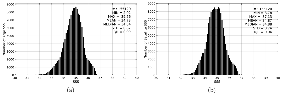
Figure 2: Histograms of SSS from Argo (a) and SMOS-L3-BEC-OA-V1-9DAYS-0.25DEG (b) considering all match-up pairs per bins of 0.1 over the Tropical Pacific Ocean Pi-MEP region and for the full satellite product period.
