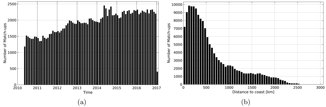
Figure 1: Number of match-ups between Argo and SMOS-L3-BEC-OA-V1-9DAYS-0.25DEG SSS as a function of time (a) and as function of the distance to coast (b) over the Tropical Pacific Ocean Pi-MEP region and for the full satellite product period.
