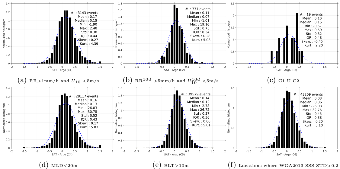
Figure 13: Normalized histogram of ΔSSS (SMOS-L3-BEC-OA-V1-9DAYS-0.25DEG - Argo) for 6 different subdatasets corresponding to: RR>1mm/h and U_{10} < 5\text{m/s} (a), RR^{10d} > 5\text{mm/h} and U_{10}^{10d} < 5\text{m/s} (b), C1 U C2 (c),MLD<20m (d),BLT>10m (e),Locations where WOA2013 SSS STD>0.2 (f).
