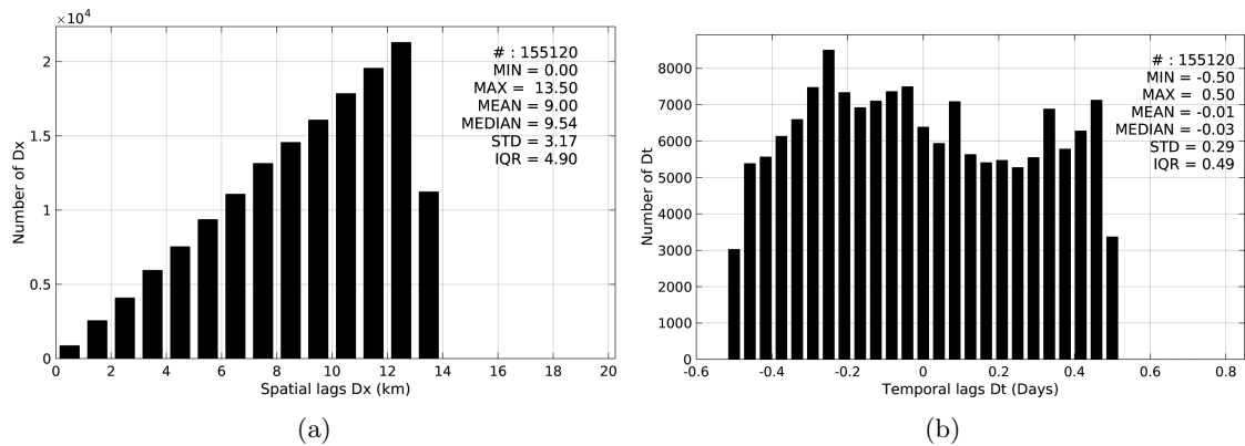
Figure 5: Histograms of the spatial (a) and temporal (b) lags between the time of the Argo measurements and the date of the corresponding SMOS-L3-BEC-OA-V1-9DAYS-0.25DEG SSS product.
