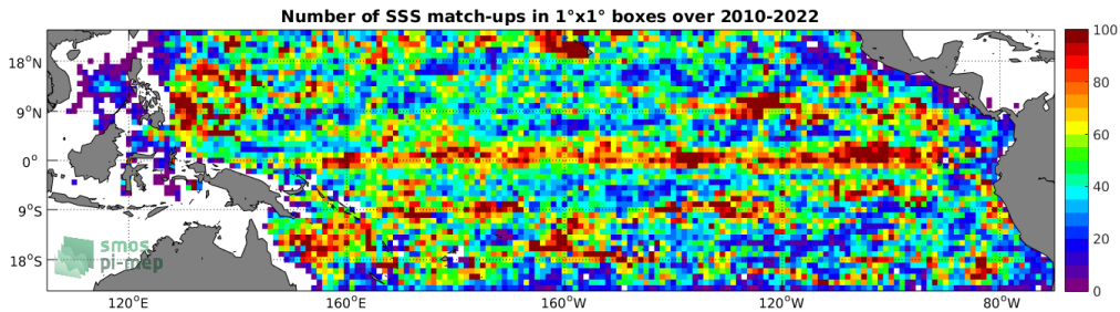
Figure 4: Number of SSS match-ups between Argo SSS and the SMOS SSS L2-AVERAGED v700 (ESA) SSS product for the Tropical Pacific Ocean Pi-MEP region over 1^\circ \times 1^\circ boxes and for the full satellite product period.
