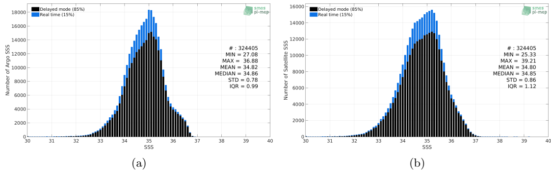
Figure 2: Histograms of SSS from Argo (a) and SMOS SSS L2-AVERAGED v700 (ESA) (b) considering all match-up pairs per bins of 0.1 over the Tropical Pacific Ocean Pi-MEP region and for the full satellite product period.
