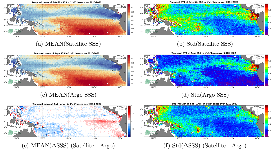
Figure 6: Temporal mean (left) and Std (right) of SSS from SMOS SSS L2-AVERAGED v700 (ESA) (top), Argo (middle), and of \Delta SSS (Satellite - Argo). Only match-up pairs are used to generate these maps.
