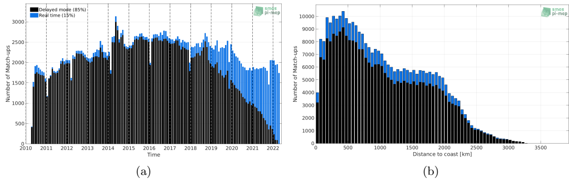
Figure 1: Number of match-ups between Argo and SMOS SSS L2-AVERAGED v700 (ESA) SSS as a function of time (a) and as function of the distance to coast (b) over the Tropical Pacific Ocean Pi-MEP region and for the full satellite product period.
