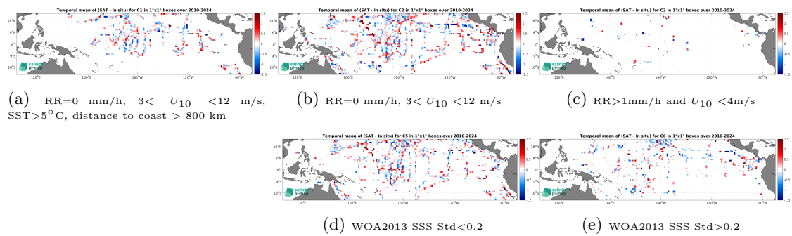
Figure 14: Temporal mean gridded over spatial boxes of size 1^\circ \times 1^\circ of \Delta SSS (SMOS SSS L2 v700 (ESA) - TSG (SAMOS)) for 5 different subdatasets corresponding to:RR=0 mm/h, 3 < U_{10} < 12 m/s, SST > 5^\circ\text{C} , distance to coast > 800 km (a), RR=0 mm/h, 3 < U_{10} < 12 m/s (b), RR > 1 mm/h and U_{10} < 4 m/s (c), WOA2013 SSS Std < 0.2 (d), WOA2013 SSS Std > 0.2 (e).
