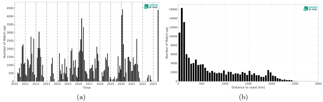
Figure 1: Number of match-ups between TSG (SAMOS) and SMOS SSS L2 v700 (ESA) SSS as a function of time (a) and as function of the distance to coast (b) over the Tropical Pacific Ocean Pi-MEP region and for the full satellite product period.
