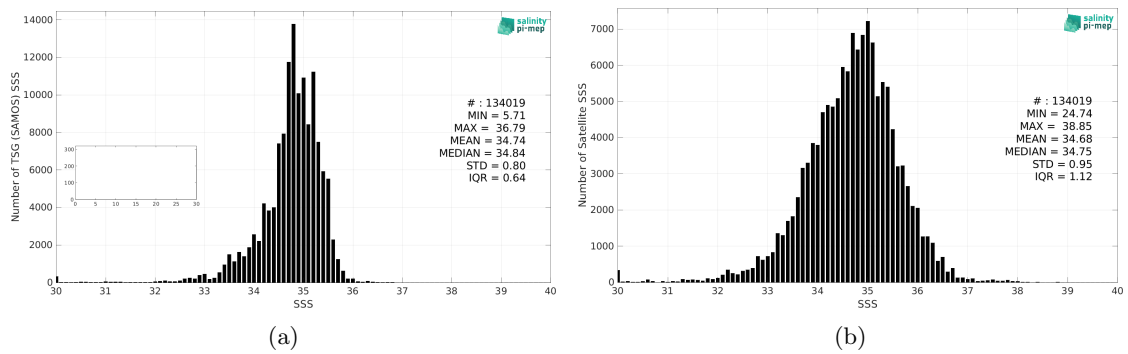
Figure 2: Histograms of SSS from TSG (SAMOS) (a) and SMOS SSS L2 v700 (ESA) (b) considering all match-up pairs per bins of 0.1 over the Tropical Pacific Ocean Pi-MEP region and for the full satellite product period.
