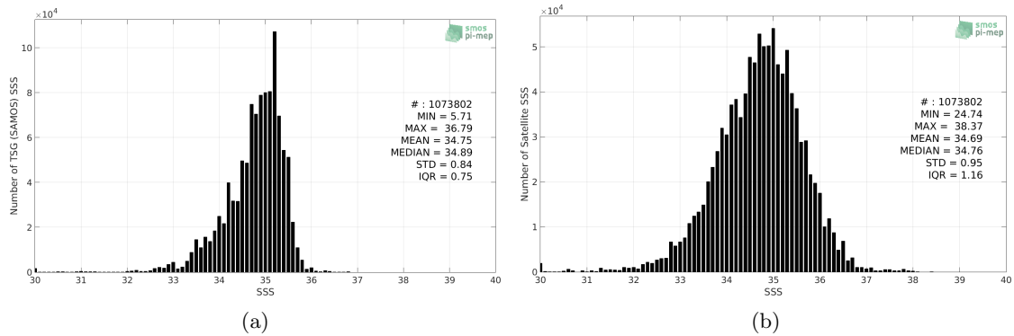
Figure 2: Histograms of SSS from TSG (SAMOS) (a) and SMOS SSS L2 v700 (ESA) (b) considering all match-up pairs per bins of 0.1 over the Tropical Pacific Ocean Pi-MEP region and for the full satellite product period.
