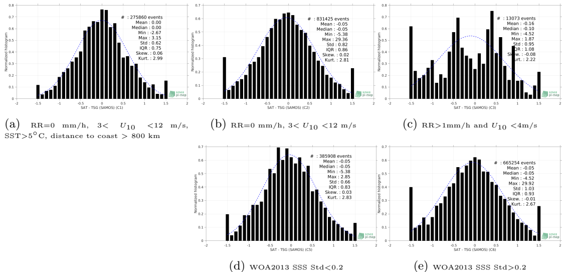
Figure 13: Normalized histogram of ΔSSS (SMOS SSS L2 v700 (ESA) - TSG (SAMOS)) for 5 different subdatasets corresponding to: RR=0 mm/h, 3 < U 10 < 12 m/s, SST>5°C, distance to coast > 800 km (a), RR=0 mm/h, 3 < U 10 < 12 m/s (b), RR>1mm/h and U 10 <4m/s (c), WOA2013 SSS Std<0.2 (d), WOA2013 SSS Std>0.2 (e).
