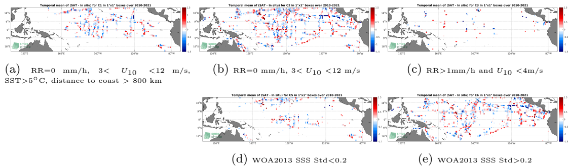
Figure 12: Temporal mean gridded over spatial boxes of size 1°x1° of ΔSSS (SMOS SSS L2 v700 (ESA) - TSG (SAMOS)) for 5 different subdatasets corresponding to:RR=0 mm/h, 3 < U 10 < 12 m/s, SST>5°C, distance to coast > 800 km (a), RR=0 mm/h, 3 < U 10 < 12 m/s (b), RR>1mm/h and U 10 <4m/s (c), WOA2013 SSS Std<0.2 (d), WOA2013 SSS Std>0.2 (e).
