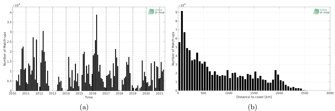
Figure 1: Number of match-ups between TSG (SAMOS) and SMOS SSS L2 v700 (ESA) SSS as a function of time (a) and as function of the distance to coast (b) over the Tropical Pacific Ocean Pi-MEP region and for the full satellite product period.
