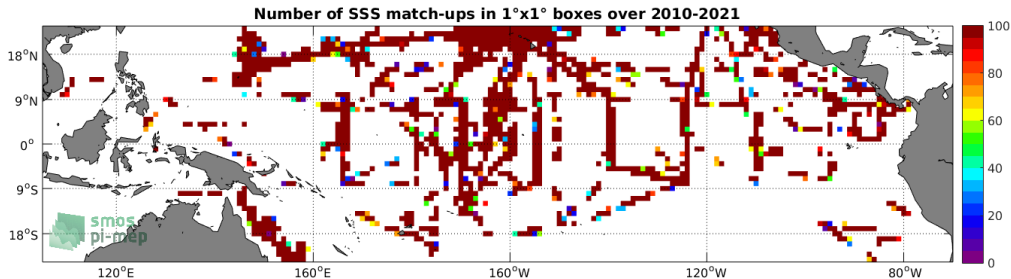
Figure 4: Number of SSS match-ups between TSG (SAMOS) SSS and the SMOS SSS L2 v700 (ESA) SSS product for the Tropical Pacific Ocean Pi-MEP region over 1^\circ \times 1^\circ boxes and for the full satellite product period.
