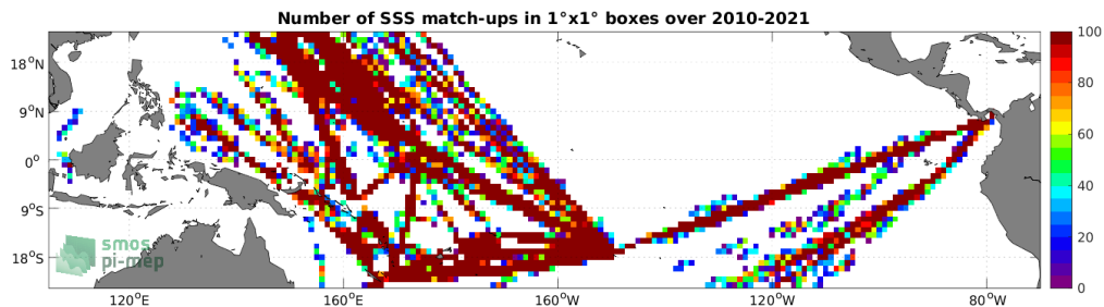
Figure 4: Number of SSS match-ups between TSG (LEGOS-DM) SSS and the SMOS SSS L2 v700 (ESA) SSS product for the Tropical Pacific Ocean Pi-MEP region over 1^\circ \times 1^\circ boxes and for the full satellite product period.
