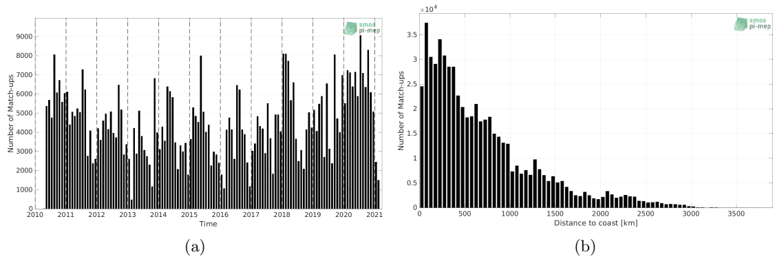
Figure 1: Number of match-ups between TSG (LEGOS-DM) and SMOS SSS L2 v700 (ESA) SSS as a function of time (a) and as function of the distance to coast (b) over the Tropical Pacific Ocean Pi-MEP region and for the full satellite product period.
