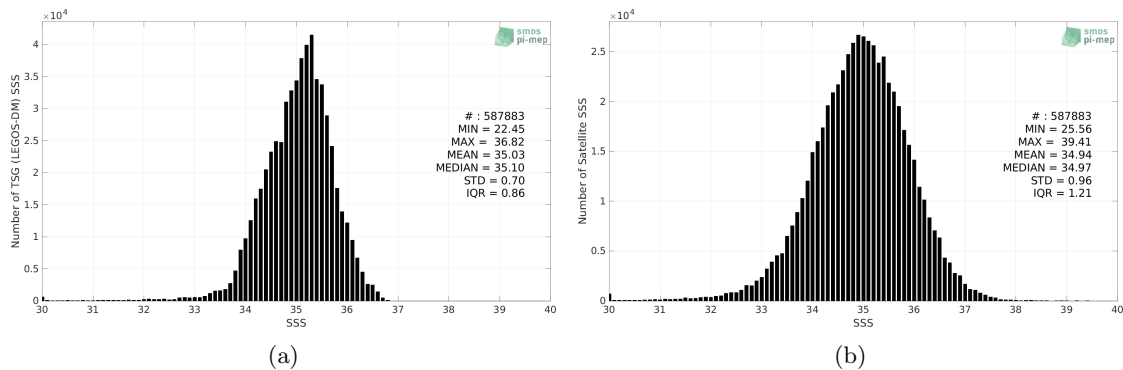
Figure 2: Histograms of SSS from TSG (LEGOS-DM) (a) and SMOS SSS L2 v700 (ESA) (b) considering all match-up pairs per bins of 0.1 over the Tropical Pacific Ocean Pi-MEP region and for the full satellite product period.
