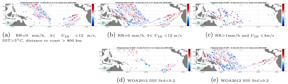
Figure 12: Temporal mean gridded over spatial boxes of size 1°x1° of \Delta SSS (SMOS SSS L2 v700 (ESA) - TSG (LEGOS-DM)) for 5 different subdatasets corresponding to:RR=0 mm/h, 3 < U_{10} < 12 m/s, SST>5°C, distance to coast > 800 km (a), RR=0 mm/h, 3 < U_{10} < 12 m/s (b), RR>1mm/h and U_{10} < 4m/s (c), WOA2013 SSS Std<0.2 (d), WOA2013 SSS Std>0.2 (e).
