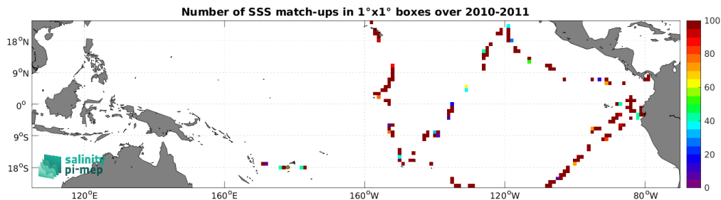
Figure 5: Number of SSS match-ups between TSG (GOSUD-Sailing-ship) SSS and the SMOS SSS L2 v700 (ESA) SSS product for the Tropical Pacific Ocean Pi-MEP region over 1^\circ \times 1^\circ boxes and for the full satellite product period.
