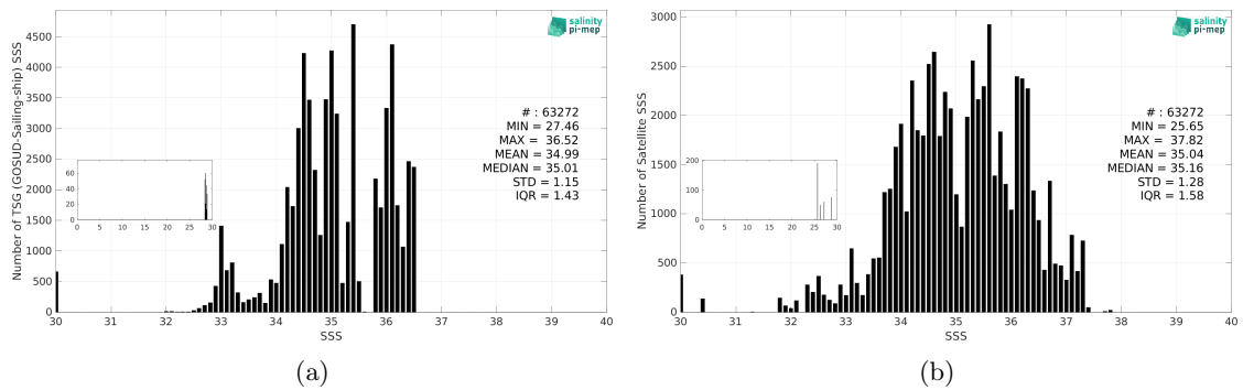
Figure 3: Histograms of SSS from TSG (GOSUD-Sailing-ship) (a) and SMOS SSS L2 v700 (ESA) (b) considering all match-up pairs per bins of 0.1 over the Tropical Pacific Ocean Pi-MEP region and for the full satellite product period.
