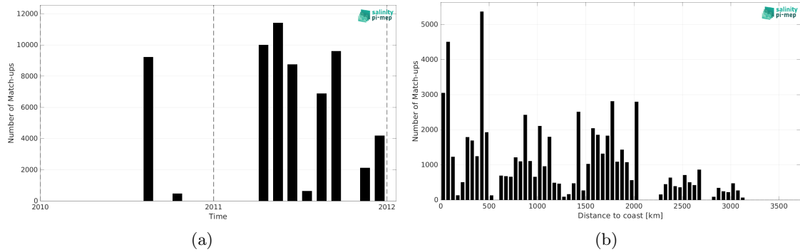
Figure 2: Number of match-ups between TSG (GOSUD-Sailing-ship) and SMOS SSS L2 v700 (ESA) SSS as a function of time (a) and as function of the distance to coast (b) over the Tropical Pacific Ocean Pi-MEP region and for the full satellite product period.
