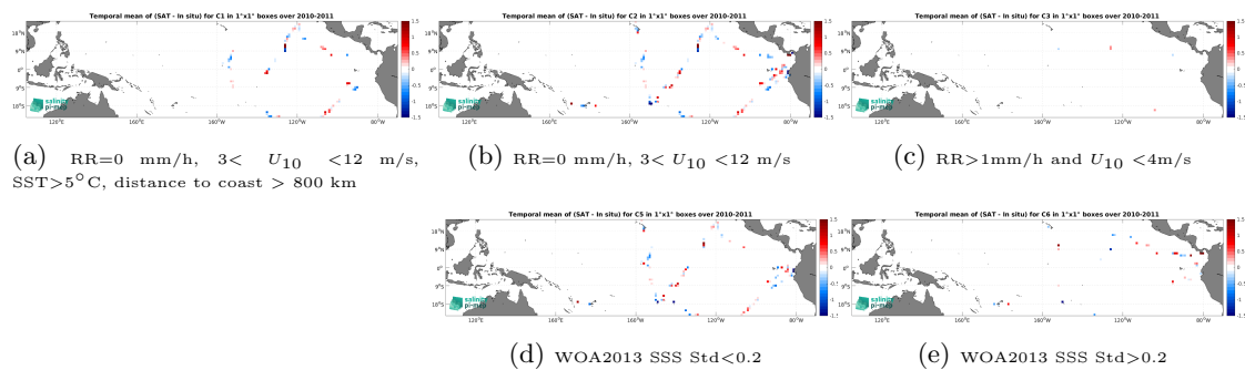
Figure 14: Temporal mean gridded over spatial boxes of size 1^\circ \times 1^\circ of \Delta\text{SSS} (SMOS SSS L2 v700 (ESA) - TSG (GOSUD-Sailing-ship)) for 5 different subdatasets corresponding to: RR=0 mm/h, 3 < U_{10} < 12 m/s, SST > 5°C, distance to coast > 800 km (a), RR=0 mm/h, 3 < U_{10} < 12 m/s (b), RR > 1mm/h and U_{10} < 4 m/s (c), WOA2013 SSS Std < 0.2 (d), WOA2013 SSS Std > 0.2 (e).
