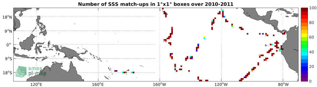
Figure 4: Number of SSS match-ups between TSG (GOSUD-Sailing-ship) SSS and the SMOS SSS L2 v700 (ESA) SSS product for the Tropical Pacific Ocean Pi-MEP region over 1^\circ \times 1^\circ boxes and for the full satellite product period.
