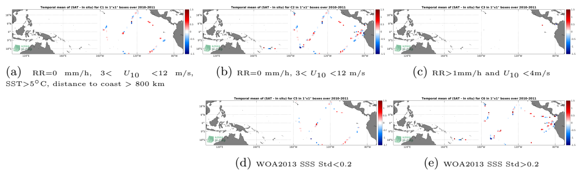
Figure 12: Temporal mean gridded over spatial boxes of size 1^\circ \times 1^\circ of \Delta\text{SSS} (SMOS SSS L2 v700 (ESA) - TSG (GOSUD-Sailing-ship)) for 5 different subdatasets corresponding to:RR=0 mm/h, 3 < U_{10} < 12 m/s, SST>5°C, distance to coast > 800 km (a), RR=0 mm/h, 3 < U_{10} < 12 m/s (b), RR>1mm/h and U_{10} < 4 m/s (c), WOA2013 SSS Std<0.2 (d), WOA2013 SSS Std>0.2 (e).
