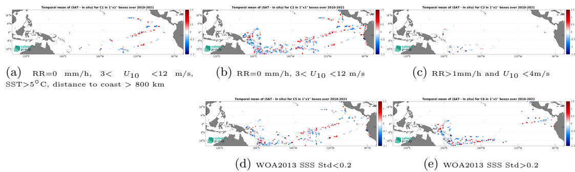
Figure 14: Temporal mean gridded over spatial boxes of size 1^\circ \times 1^\circ of \Delta SSS (SMOS SSS L2 v700 (ESA) - TSG (GOSUD-Research-vessel)) for 5 different subdatasets corresponding to:RR=0 mm/h, 3 < U_{10} < 12 m/s, SST > 5°C, distance to coast > 800 km (a), RR=0 mm/h, 3 < U_{10} < 12 m/s (b), RR > 1mm/h and U_{10} < 4 m/s (c), WOA2013 SSS Std < 0.2 (d), WOA2013 SSS Std > 0.2 (e).
