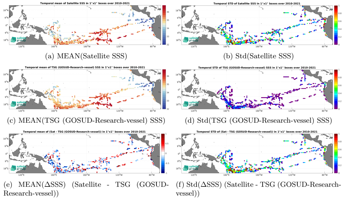
Figure 7: Temporal mean (left) and Std (right) of SSS from SMOS SSS L2 v700 (ESA) (top), TSG (GOSUD-Research-vessel) (middle), and of \Delta SSS (Satellite - TSG (GOSUD-Research-vessel)). Only match-up pairs are used to generate these maps.
