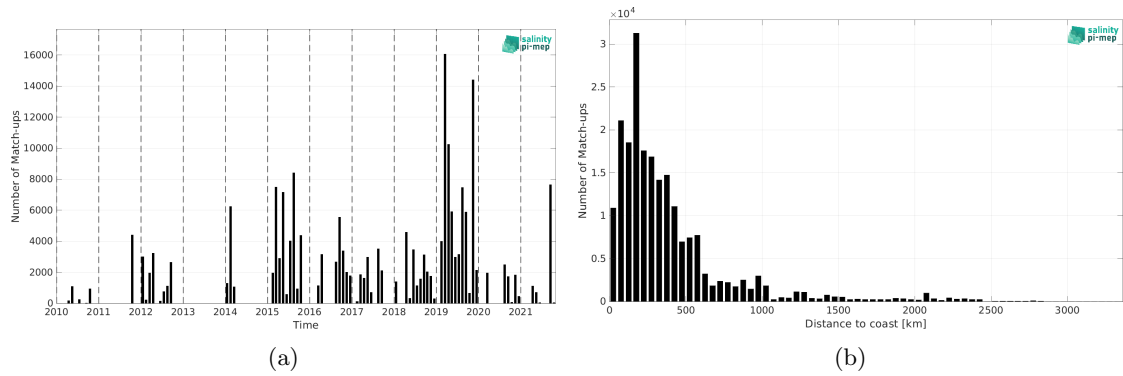
Figure 2: Number of match-ups between TSG (GOSUD-Research-vessel) and SMOS SSS L2 v700 (ESA) SSS as a function of time (a) and as function of the distance to coast (b) over the Tropical Pacific Ocean Pi-MEP region and for the full satellite product period.
