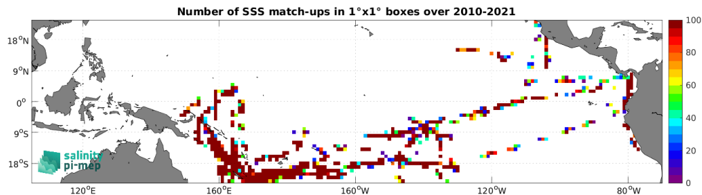
Figure 5: Number of SSS match-ups between TSG (GOSUD-Research-vessel) SSS and the SMOS SSS L2 v700 (ESA) SSS product for the Tropical Pacific Ocean Pi-MEP region over 1^\circ \times 1^\circ boxes and for the full satellite product period.
