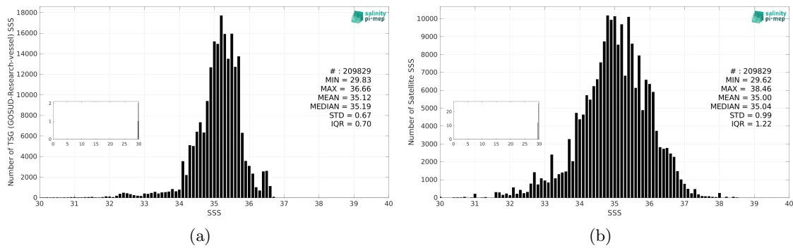
Figure 3: Histograms of SSS from TSG (GOSUD-Research-vessel) (a) and SMOS SSS L2 v700 (ESA) (b) considering all match-up pairs per bins of 0.1 over the Tropical Pacific Ocean Pi-MEP region and for the full satellite product period.
