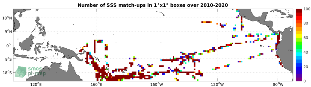
Figure 4: Number of SSS match-ups between TSG (GOSUD-Research-vessel) SSS and the SMOS SSS L2 v700 (ESA) SSS product for the Tropical Pacific Ocean Pi-MEP region over 1^\circ \times 1^\circ boxes and for the full satellite product period.
