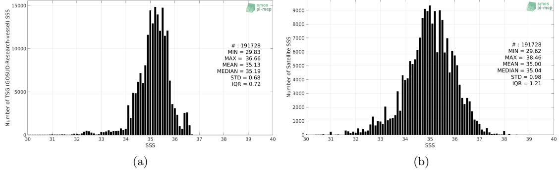
Figure 2: Histograms of SSS from TSG (GOSUD-Research-vessel) (a) and SMOS SSS L2 v700 (ESA) (b) considering all match-up pairs per bins of 0.1 over the Tropical Pacific Ocean Pi-MEP region and for the full satellite product period.
