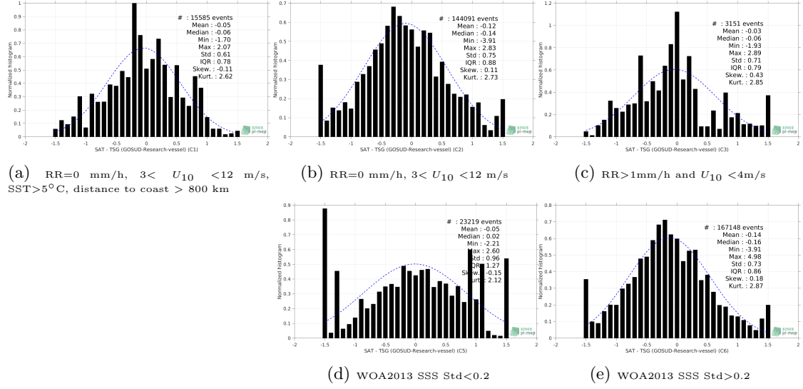
Figure 13: Normalized histogram of \Delta SSS (SMOS SSS L2 v700 (ESA) - TSG (GOSUD-Research-vessel)) for 5 different subdatasets corresponding to: RR=0 mm/h, 3 < U_{10} < 12 m/s, SST>5°C, distance to coast > 800 km (a), RR=0 mm/h, 3 < U_{10} < 12 m/s (b), RR>1mm/h and U_{10} < 4 m/s (c), WOA2013 SSS Std<0.2 (d), WOA2013 SSS Std>0.2 (e).
