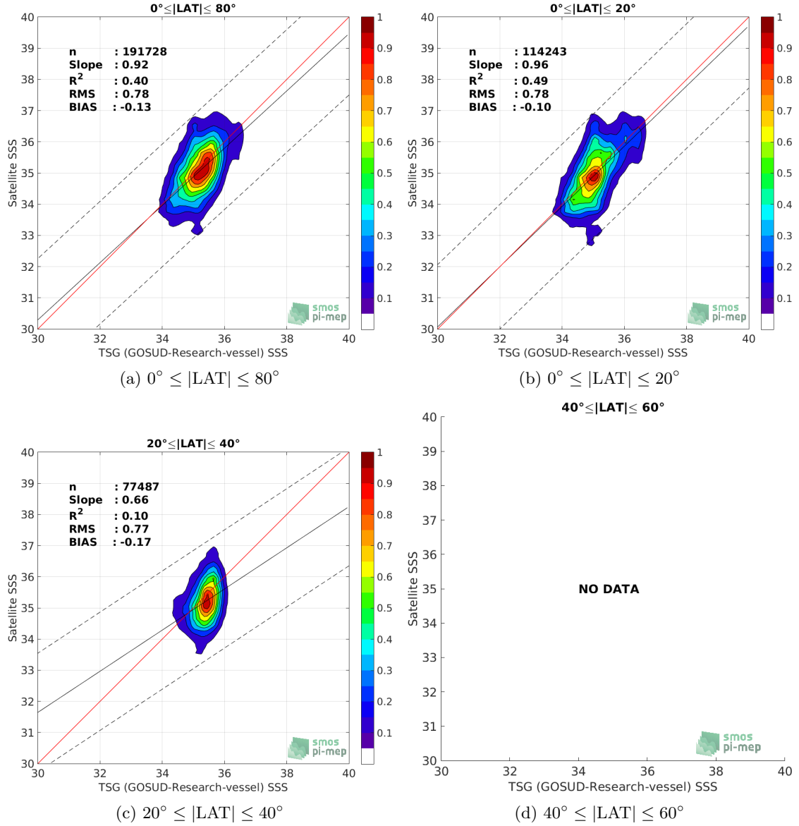
Figure 9: Contour maps of the concentration of SMOS SSS L2 v700 (ESA) SSS (y-axis) versus TSG (GOSUD-Research-vessel) SSS (x-axis) at match-up pairs for different latitude bands. For each plot, the red line shows x=y . The black thin and dashed lines indicate a linear fit through the data cloud and the \pm 95\% confidence levels, respectively. The number match-up pairs n , the slope and R^2 coefficient of the linear fit, the root mean square (RMS) and the mean bias between satellite and in situ data are indicated for each latitude band in each plots.
