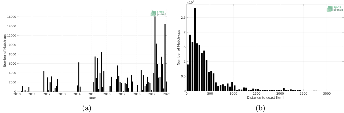
Figure 1: Number of match-ups between TSG (GOSUD-Research-vessel) and SMOS SSS L2 v700 (ESA) SSS as a function of time (a) and as function of the distance to coast (b) over the Tropical Pacific Ocean Pi-MEP region and for the full satellite product period.
