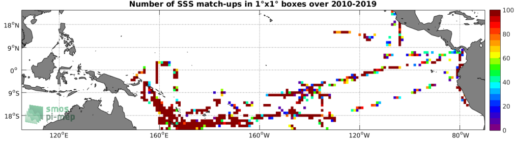
Figure 4: Number of SSS match-ups between TSG (GOSUD-Research-vessel) SSS and the SMOS SSS L2 v700 (ESA) SSS product for the Tropical Pacific Ocean Pi-MEP region over 1^\circ \times 1^\circ boxes and for the full satellite product period.
