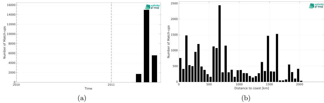
Figure 2: Number of match-ups between TSG (CSIC-UTM) and SMOS SSS L2 v700 (ESA) SSS as a function of time (a) and as function of the distance to coast (b) over the Tropical Pacific Ocean Pi-MEP region and for the full satellite product period.
