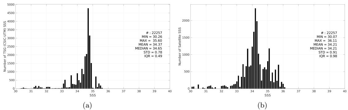
Figure 3: Histograms of SSS from TSG (CSIC-UTM) (a) and SMOS SSS L2 v700 (ESA) (b) considering all match-up pairs per bins of 0.1 over the Tropical Pacific Ocean Pi-MEP region and for the full satellite product period.
