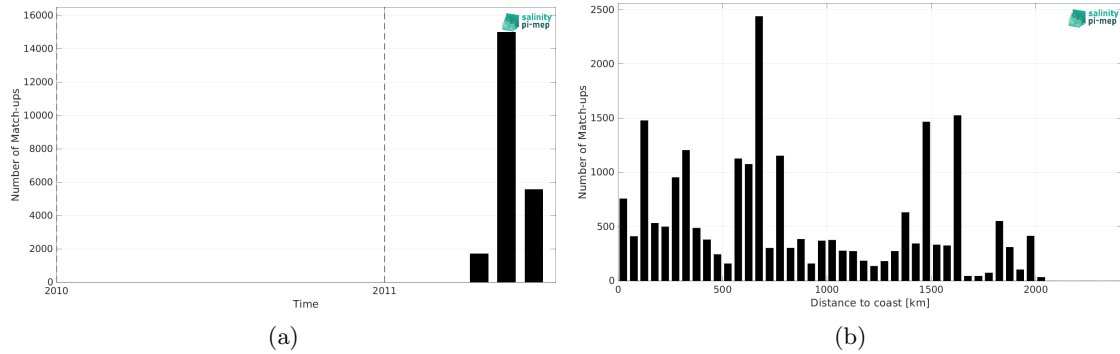
Figure 1: Number of match-ups between TSG (CSIC-UTM) and SMOS SSS L2 v700 (ESA) SSS as a function of time (a) and as function of the distance to coast (b) over the Tropical Pacific Ocean Pi-MEP region and for the full satellite product period.
