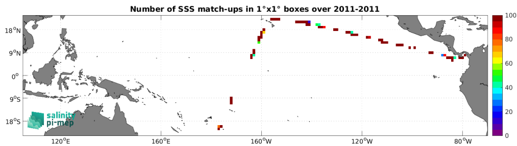
Figure 4: Number of SSS match-ups between TSG (CSIC-UTM) SSS and the SMOS SSS L2 v700 (ESA) SSS product for the Tropical Pacific Ocean Pi-MEP region over 1^\circ \times 1^\circ boxes and for the full satellite product period.
