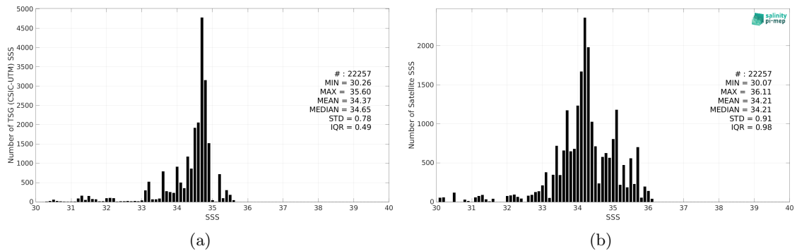
Figure 2: Histograms of SSS from TSG (CSIC-UTM) (a) and SMOS SSS L2 v700 (ESA) (b) considering all match-up pairs per bins of 0.1 over the Tropical Pacific Ocean Pi-MEP region and for the full satellite product period.
