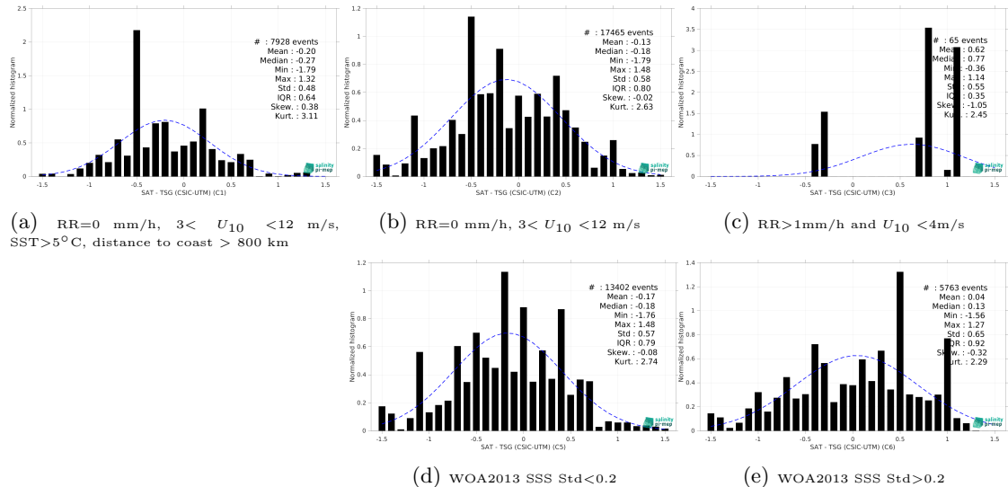
Figure 13: Normalized histogram of \Delta SSS (SMOS SSS L2 v700 (ESA) - TSG (CSIC-UTM)) for 5 different subdatasets corresponding to: RR=0 mm/h, 3 < U_{10} < 12 m/s, SST >5^\circ\text{C} , distance to coast > 800 km (a), RR=0 mm/h, 3 < U_{10} < 12 m/s (b), RR >1 mm/h and U_{10} < 4 m/s (c), WOA2013 SSS Std <0.2 (d), WOA2013 SSS Std >0.2 (e).
