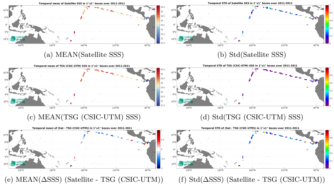
Figure 6: Temporal mean (left) and Std (right) of SSS from SMOS SSS L2 v700 (ESA) (top), TSG (CSIC-UTM) (middle), and of \Delta SSS (Satellite - TSG (CSIC-UTM)). Only match-up pairs are used to generate these maps.
