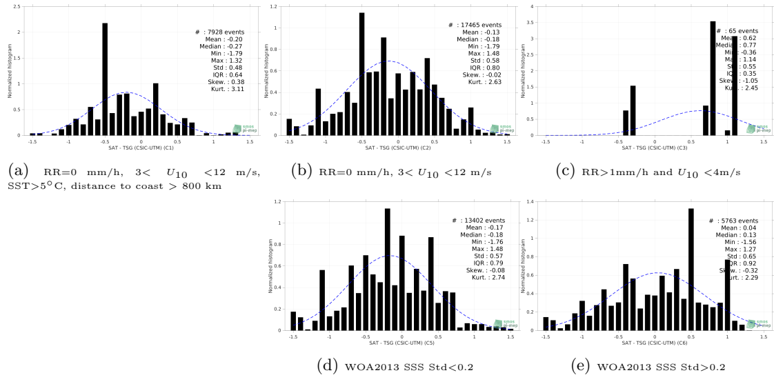
Figure 13: Normalized histogram of \Delta SSS (SMOS SSS L2 v700 (ESA) - TSG (CSIC-UTM)) for 5 different subdatasets corresponding to: RR=0 mm/h, 3 < U_{10} < 12 m/s, SST >5^\circ\text{C} , distance to coast > 800 km (a), RR=0 mm/h, 3 < U_{10} < 12 m/s (b), RR >1 mm/h and U_{10} < 4 m/s (c), WOA2013 SSS Std <0.2 (d), WOA2013 SSS Std >0.2 (e).
