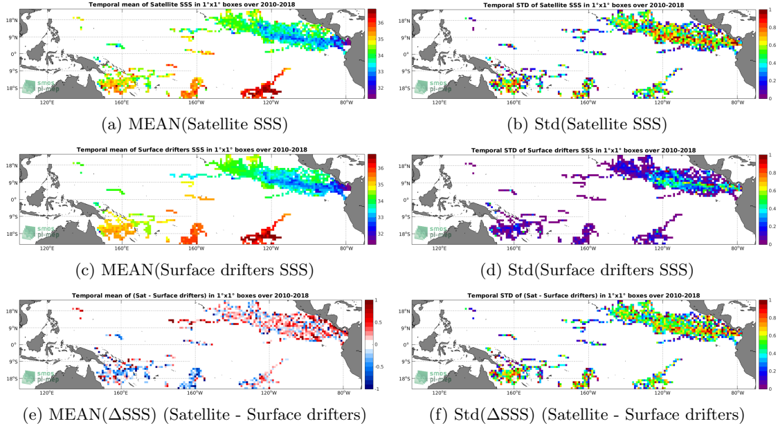
Figure 5: Temporal mean (left) and Std (right) of SSS from SMOS SSS L2 v700 (ESA) (top), Surface drifters (middle), and of \Delta SSS (Satellite - Surface drifters). Only match-up pairs are used to generate these maps.
