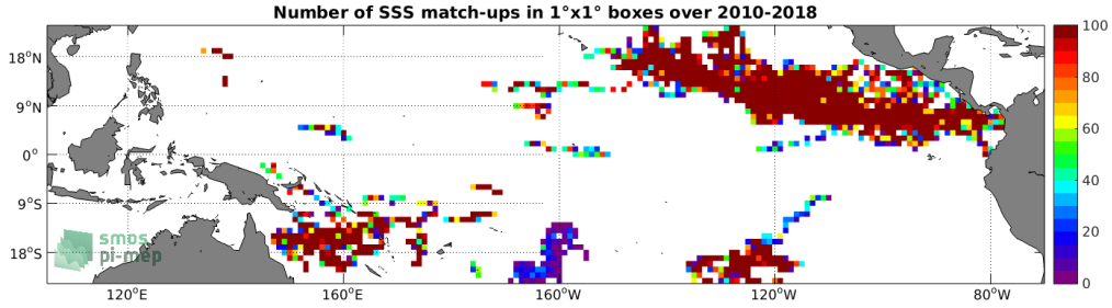
Figure 3: Number of SSS match-ups between Surface drifters SSS and the SMOS SSS L2 v700 (ESA) SSS product for the Tropical Pacific Ocean Pi-MEP region over 1^\circ \times 1^\circ boxes and for the full satellite product period.
