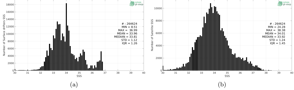
Figure 2: Histograms of SSS from Surface drifters (a) and SMOS SSS L2 v700 (ESA) (b) considering all match-up pairs per bins of 0.1 over the Tropical Pacific Ocean Pi-MEP region and for the full satellite product period.
