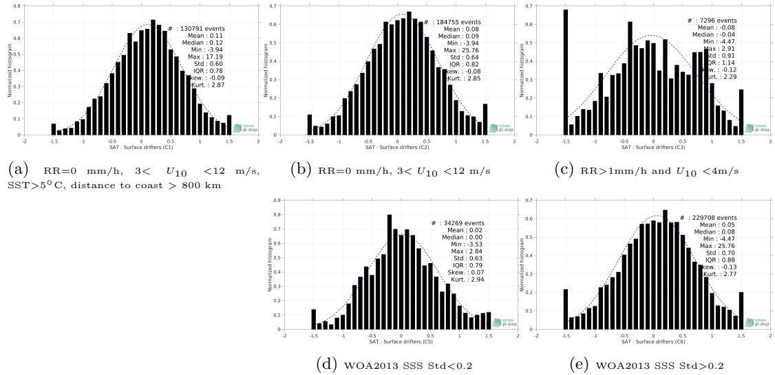
Figure 12: Normalized histogram of \Delta SSS (SMOS SSS L2 v700 (ESA) - Surface drifters) for 5 different subdatasets corresponding to: RR=0 mm/h, 3 < U_{10} < 12 m/s, SST >5^\circ\text{C} , distance to coast > 800 km (a), RR=0 mm/h, 3 < U_{10} < 12 m/s (b), RR >1 mm/h and U_{10} <4 m/s (c), WOA2013 SSS Std <0.2 (d), WOA2013 SSS Std >0.2 (e).
