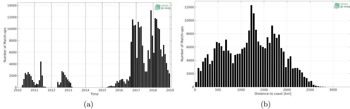
Figure 1: Number of match-ups between Surface drifters and SMOS SSS L2 v700 (ESA) SSS as a function of time (a) and as function of the distance to coast (b) over the Tropical Pacific Ocean Pi-MEP region and for the full satellite product period.
