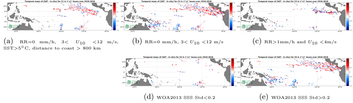
Figure 11: Temporal mean gridded over spatial boxes of size 1^\circ \times 1^\circ of \Delta SSS (SMOS SSS L2 v700 (ESA) - Surface drifters) for 5 different subdatasets corresponding to: RR=0 mm/h, 3 < U_{10} < 12 m/s, SST >5^\circ\text{C} , distance to coast > 800 km (a), RR=0 mm/h, 3 < U_{10} < 12 m/s (b), RR >1 mm/h and U_{10} <4 m/s (c), WOA2013 SSS Std <0.2 (d), WOA2013 SSS Std >0.2 (e).
