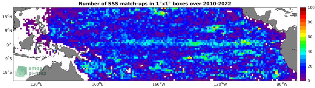
Figure 4: Number of SSS match-ups between Argo SSS and the SMOS SSS L2 v700 (ESA) SSS product for the Tropical Pacific Ocean Pi-MEP region over 1^\circ \times 1^\circ boxes and for the full satellite product period.
