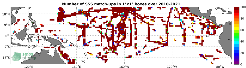
Figure 4: Number of SSS match-ups between TSG (SAMOS) SSS and the SMOS SSS L2 v662 (ESA) SSS product for the Tropical Pacific Ocean Pi-MEP region over 1^\circ \times 1^\circ boxes and for the full satellite product period.
