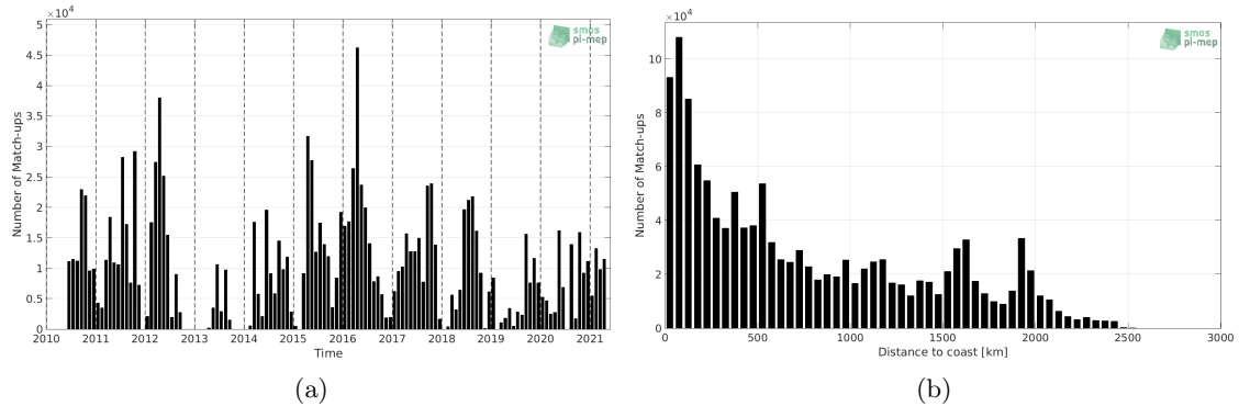
Figure 1: Number of match-ups between TSG (SAMOS) and SMOS SSS L2 v662 (ESA) SSS as a function of time (a) and as function of the distance to coast (b) over the Tropical Pacific Ocean Pi-MEP region and for the full satellite product period.
