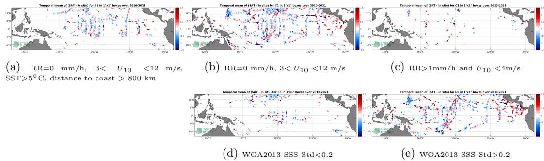
Figure 12: Temporal mean gridded over spatial boxes of size 1°x1° of ΔSSS (SMOS SSS L2 v662 (ESA) - TSG (SAMOS)) for 5 different subdatasets corresponding to:RR=0 mm/h, 3 < U 10 < 12 m/s, SST>5°C, distance to coast > 800 km (a), RR=0 mm/h, 3 < U 10 < 12 m/s (b), RR>1mm/h and U 10 < 4m/s (c), WOA2013 SSS Std<0.2 (d), WOA2013 SSS Std>0.2 (e).
