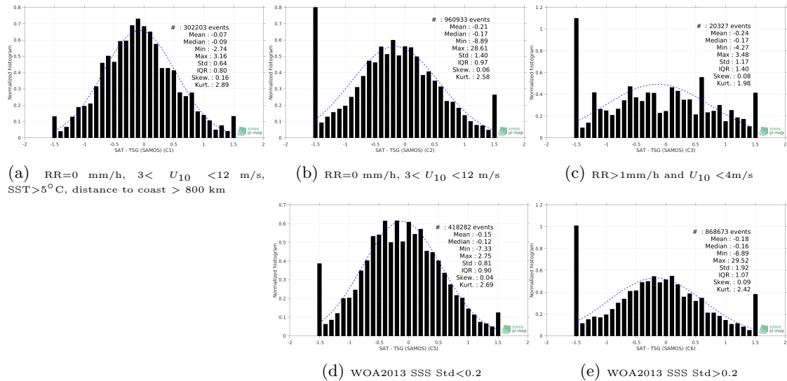
Figure 13: Normalized histogram of ΔSSS (SMOS SSS L2 v662 (ESA) - TSG (SAMOS)) for 5 different subdatasets corresponding to: RR=0 mm/h, 3 < U 10 < 12 m/s, SST>5°C, distance to coast > 800 km (a), RR=0 mm/h, 3 < U 10 < 12 m/s (b), RR>1mm/h and U 10 < 4m/s (c), WOA2013 SSS Std<0.2 (d), WOA2013 SSS Std>0.2 (e).
