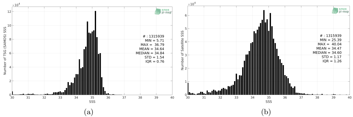
Figure 2: Histograms of SSS from TSG (SAMOS) (a) and SMOS SSS L2 v662 (ESA) (b) considering all match-up pairs per bins of 0.1 over the Tropical Pacific Ocean Pi-MEP region and for the full satellite product period.
