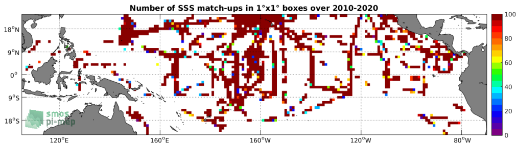
Figure 4: Number of SSS match-ups between TSG (SAMOS) SSS and the SMOS SSS L2 v662 (ESA) SSS product for the Tropical Pacific Ocean Pi-MEP region over 1°x1° boxes and for the full satellite product period.
