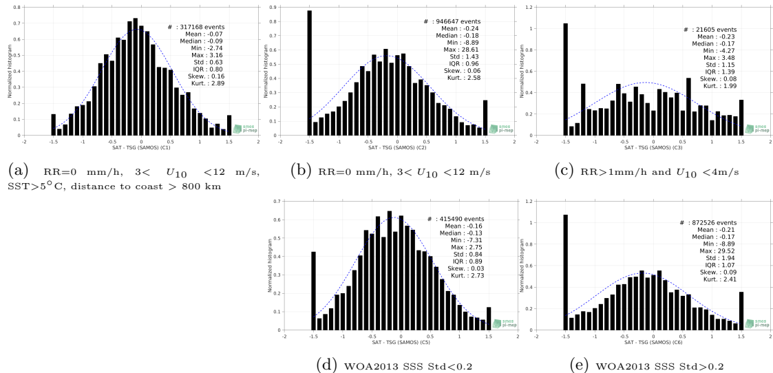
Figure 13: Normalized histogram of ΔSSS (SMOS SSS L2 v662 (ESA) - TSG (SAMOS)) for 5 different subdatasets corresponding to: RR=0 mm/h, 3 < U 10 < 12 m/s, SST>5°C, distance to coast > 800 km (a), RR=0 mm/h, 3 < U 10 < 12 m/s (b), RR>1mm/h and U 10 <4m/s (c), WOA2013 SSS Std<0.2 (d), WOA2013 SSS Std>0.2 (e).
