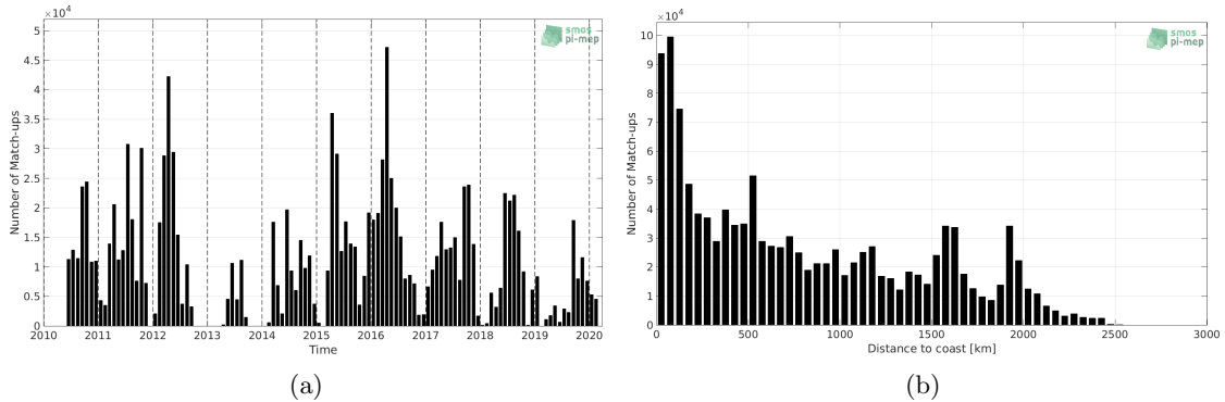
Figure 1: Number of match-ups between TSG-SAMOS and SMOS L2 v662 (ESA) SSS as a function of time (a) and as function of the distance to coast (b) over the Tropical Pacific Ocean Pi-MEP region and for the full satellite product period.
