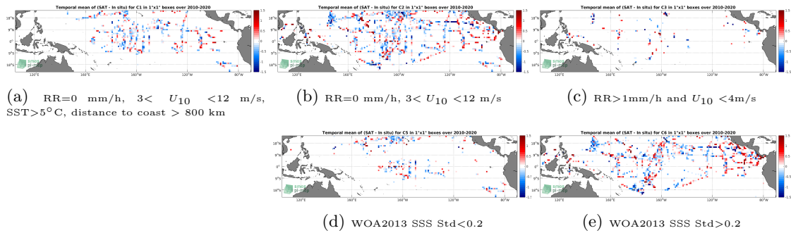
Figure 12: Temporal mean gridded over spatial boxes of size 1°x1° of ΔSSS (SMOS L2 v662 (ESA) - TSG-SAMOS) for 5 different subdatasets corresponding to:RR=0 mm/h, 3 < U 10 < 12 m/s, SST>5°C, distance to coast > 800 km (a), RR=0 mm/h, 3 < U 10 < 12 m/s (b), RR>1mm/h and U 10 < 4m/s (c), WOA2013 SSS Std<0.2 (d), WOA2013 SSS Std>0.2 (e).
