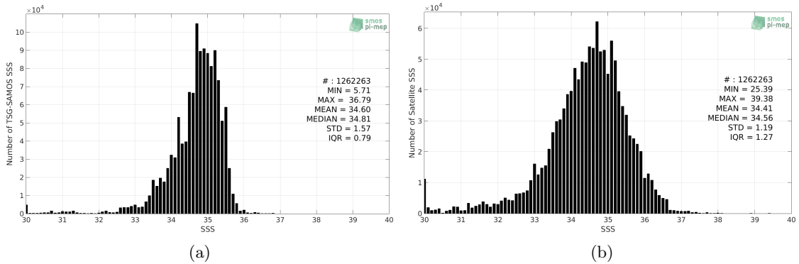
Figure 2: Histograms of SSS from TSG-SAMOS (a) and SMOS L2 v662 (ESA) (b) considering all match-up pairs per bins of 0.1 over the Tropical Pacific Ocean Pi-MEP region and for the full satellite product period.
