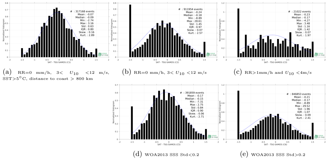
Figure 13: Normalized histogram of ΔSSS (SMOS L2 v662 (ESA) - TSG-SAMOS) for 5 different subdatasets corresponding to: RR=0 mm/h, 3 < U 10 < 12 m/s, SST>5°C, distance to coast > 800 km (a), RR=0 mm/h, 3 < U 10 < 12 m/s (b), RR>1mm/h and U 10 < 4m/s (c), WOA2013 SSS Std<0.2 (d), WOA2013 SSS Std>0.2 (e).
