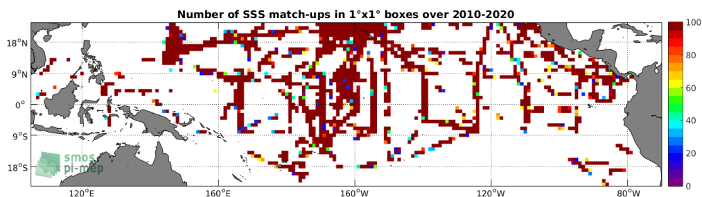
Figure 4: Number of SSS match-ups between TSG-SAMOS SSS and the SMOS L2 v662 (ESA) SSS product for the Tropical Pacific Ocean Pi-MEP region over 1^\circ \times 1^\circ boxes and for the full satellite product period.
