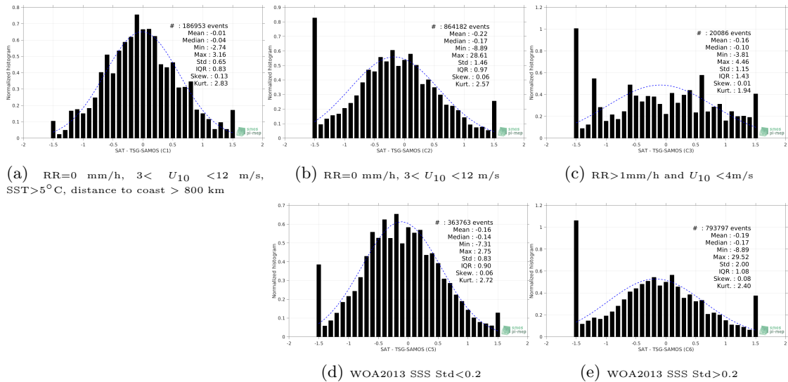
Figure 13: Normalized histogram of \Delta SSS (SMOS-L2-DPGS-v662 - TSG-SAMOS) for 5 different subdatasets corresponding to: RR=0 mm/h, 3 < U_{10} < 12 m/s, SST >5^\circ C, distance to coast > 800 km (a), RR=0 mm/h, 3 < U_{10} < 12 m/s (b), RR >1 mm/h and U_{10} < 4 m/s (c), WOA2013 SSS Std <0.2 (d), WOA2013 SSS Std >0.2 (e).
