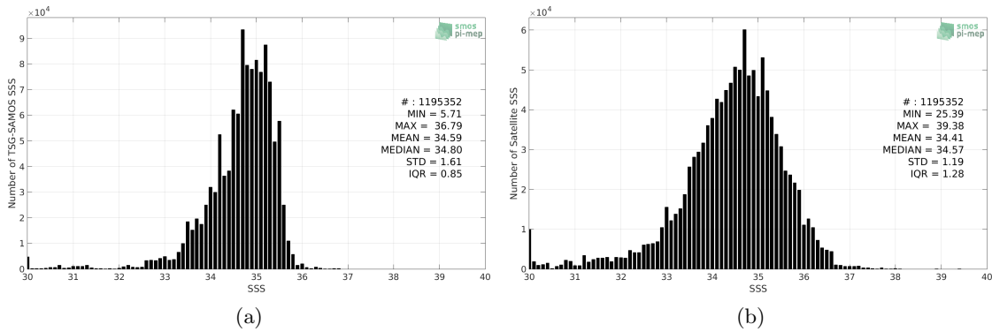
Figure 2: Histograms of SSS from TSG-SAMOS (a) and SMOS-L2-DPGS-v662 (b) considering all match-up pairs per bins of 0.1 over the Tropical Pacific Ocean Pi-MEP region and for the full satellite product period.
