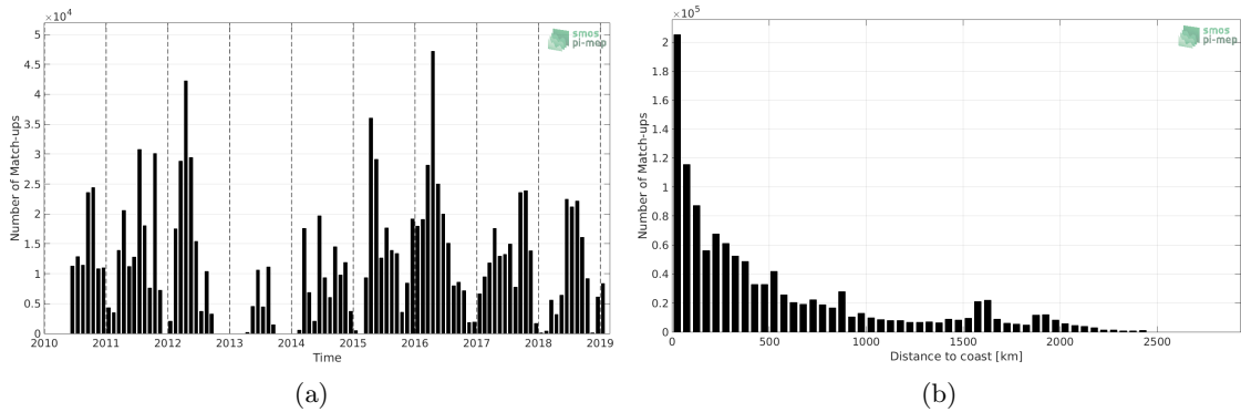
Figure 1: Number of match-ups between TSG-SAMOS and SMOS-L2-DPGS-v662 SSS as a function of time (a) and as function of the distance to coast (b) over the Tropical Pacific Ocean Pi-MEP region and for the full satellite product period.
