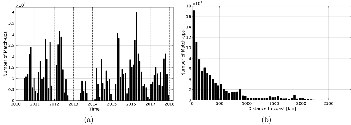
Figure 1: Number of match-ups between TSG-SAMOS and SMOS-L2-DPGS-v662 SSS as a function of time (a) and as function of the distance to coast (b) over the Tropical Pacific Ocean Pi-MEP region and for the full satellite product period.
