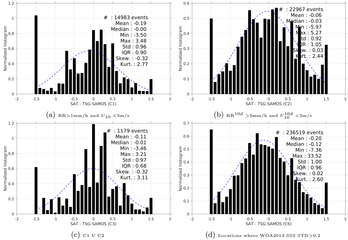
Figure 13: Normalized histogram of \Delta\text{SSS} (SMOS-L2-DPGS-v662 - TSG-SAMOS) for 6 different subdatasets corresponding to: \text{RR} > 1\text{mm/h} and U_{10} < 5\text{m/s} (a), \text{RR}^{10d} > 5\text{mm/h} and U_{10}^{10d} < 5\text{m/s} (b), C1 \cup C2 (c), Locations where WOA2013 SSS STD > 0.2 (d).
