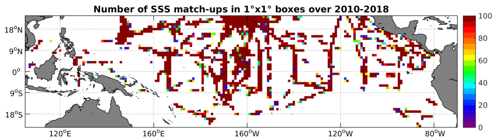
Figure 4: Number of SSS match-ups between TSG-SAMOS SSS and the SMOS-L2-DPGS-v662 SSS product for the Tropical Pacific Ocean Pi-MEP region over 1^\circ \times 1^\circ boxes and for the full satellite product period.
