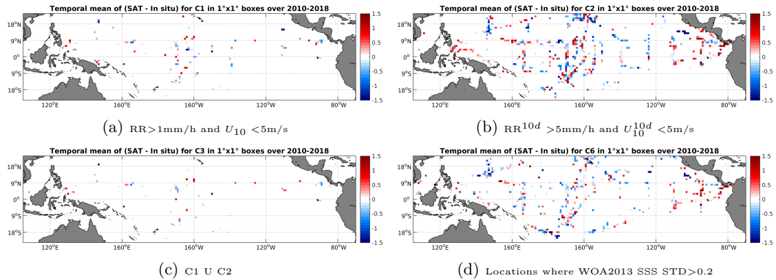
Figure 12: Temporal mean gridded over spatial boxes of size 1^\circ \times 1^\circ of \Delta SSS (SMOS-L2-DPGS-v662 - TSG-SAMOS) for 4 different subdatasets corresponding to: RR > 1\text{mm/h} and U_{10} < 5\text{m/s} (a), RR^{10d} > 5\text{mm/h} and U_{10}^{10d} < 5\text{m/s} (b), C1 U C2 (c), Locations where WOA2013 SSS STD > 0.2 (d).
