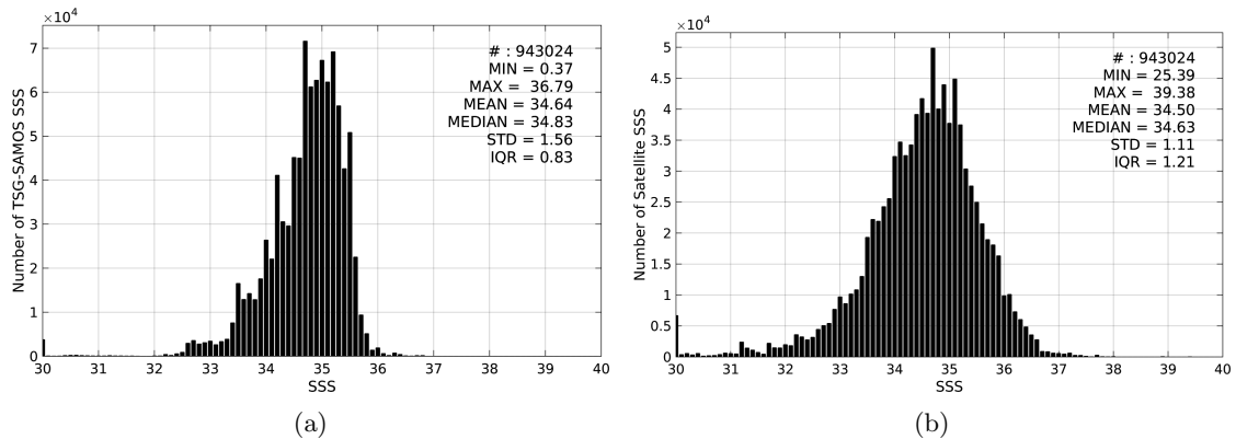
Figure 2: Histograms of SSS from TSG-SAMOS (a) and SMOS-L2-DPGS-v662 (b) considering all match-up pairs per bins of 0.1 over the Tropical Pacific Ocean Pi-MEP region and for the full satellite product period.
