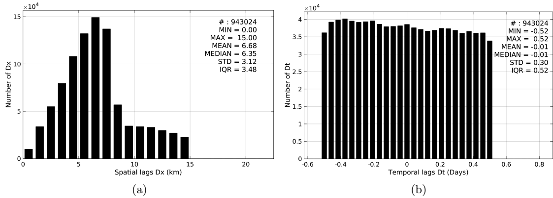
Figure 5: Histograms of the spatial (a) and temporal (b) lags between the time of the TSG-SAMOS measurements and the date of the corresponding SMOS-L2-DPGS-v662 SSS product.
