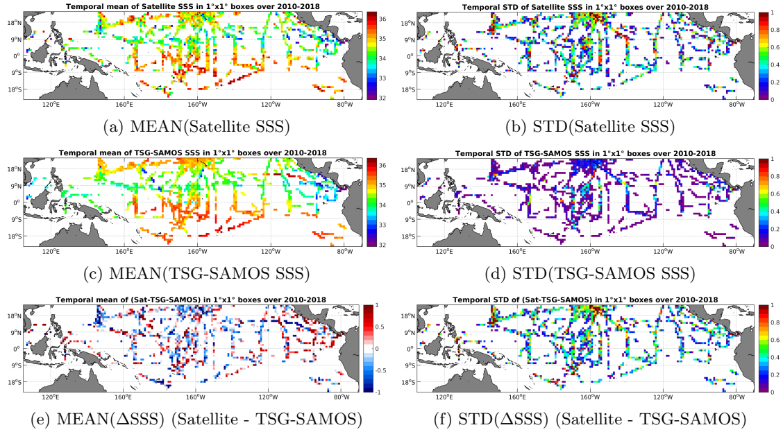
Figure 6: Temporal mean (left) and STD (right) of SSS from SMOS-L2-DPGS-v662 (top), TSG-SAMOS (middle), and of \Delta SSS (Satellite - TSG-SAMOS). Only match-up pairs are used to generate these maps.
