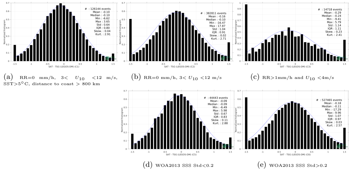
Figure 13: Normalized histogram of \Delta SSS (SMOS SSS L2 v662 (ESA) - TSG (LEGOS-DM)) for 5 different subdatasets corresponding to: RR=0 mm/h, 3< U_{10} <12 m/s, SST>5°C, distance to coast > 800 km (a), RR=0 mm/h, 3< U_{10} <12 m/s (b), RR>1mm/h and U_{10} <4m/s (c), WOA2013 SSS Std<0.2 (d), WOA2013 SSS Std>0.2 (e).
