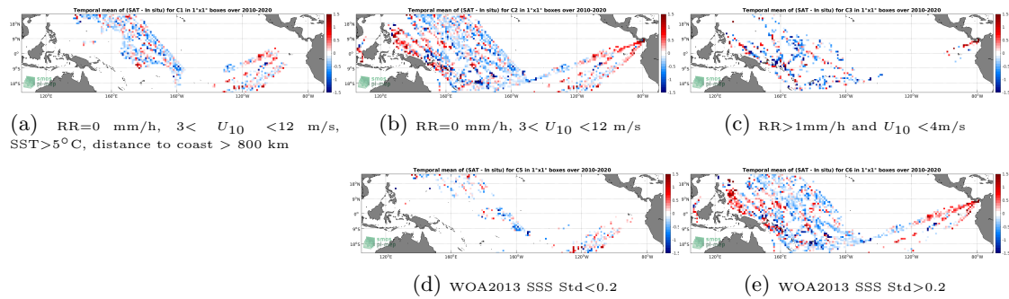
Figure 12: Temporal mean gridded over spatial boxes of size 1°x1° of \Delta SSS (SMOS SSS L2 v662 (ESA) - TSG (LEGOS-DM)) for 5 different subdatasets corresponding to:RR=0 mm/h, 3< U_{10} <12 m/s, SST>5°C, distance to coast > 800 km (a), RR=0 mm/h, 3< U_{10} <12 m/s (b), RR>1mm/h and U_{10} <4m/s (c), WOA2013 SSS Std<0.2 (d), WOA2013 SSS Std>0.2 (e).
