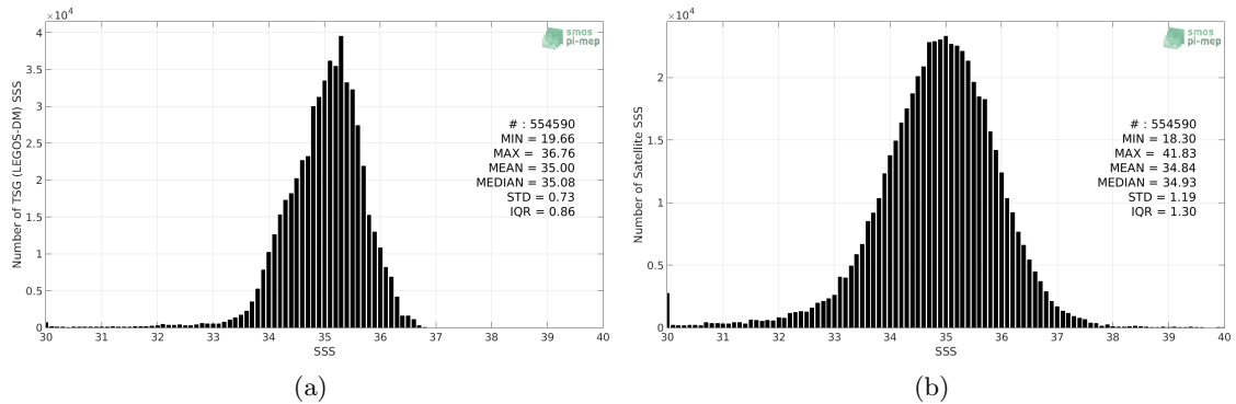
Figure 2: Histograms of SSS from TSG (LEGOS-DM) (a) and SMOS SSS L2 v662 (ESA) (b) considering all match-up pairs per bins of 0.1 over the Tropical Pacific Ocean Pi-MEP region and for the full satellite product period.
