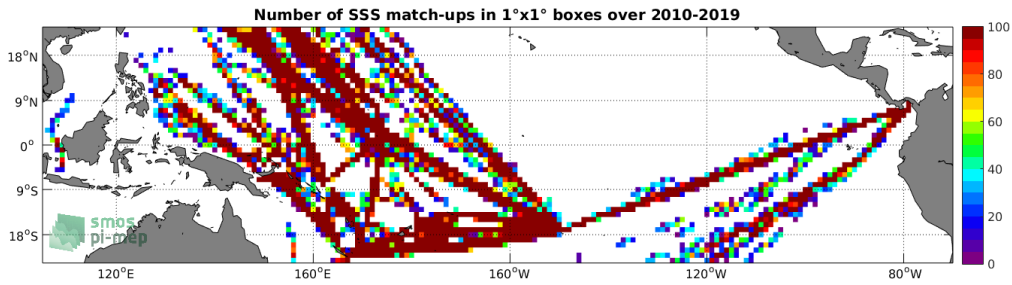
Figure 4: Number of SSS match-ups between TSG (LEGOS-DM) SSS and the SMOS SSS L2 v662 (ESA) SSS product for the Tropical Pacific Ocean Pi-MEP region over 1°x1° boxes and for the full satellite product period.
