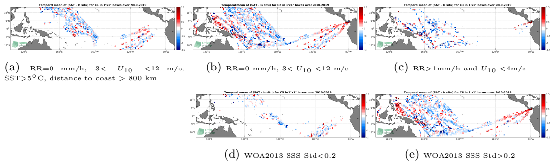
Figure 12: Temporal mean gridded over spatial boxes of size 1°x1° of ΔSSS (SMOS SSS L2 v662 (ESA) - TSG (LEGOS-DM)) for 5 different subdatasets corresponding to:RR=0 mm/h, 3 < U_{10} < 12 m/s, SST>5°C, distance to coast > 800 km (a), RR=0 mm/h, 3 < U_{10} < 12 m/s (b), RR>1mm/h and U_{10} < 4m/s (c), WOA2013 SSS Std<0.2 (d), WOA2013 SSS Std>0.2 (e).
