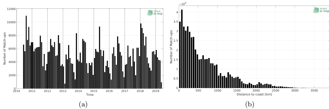
Figure 1: Number of match-ups between TSG (LEGOS-DM) and SMOS SSS L2 v662 (ESA) SSS as a function of time (a) and as function of the distance to coast (b) over the Tropical Pacific Ocean Pi-MEP region and for the full satellite product period.
