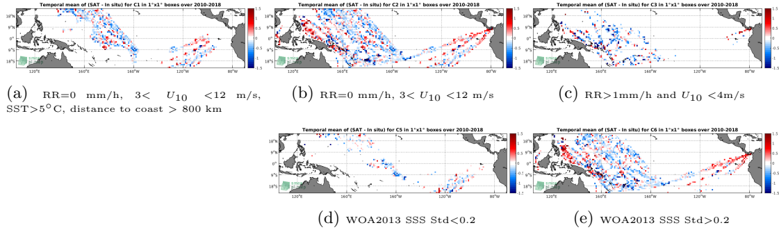
Figure 12: Temporal mean gridded over spatial boxes of size 1°x1° of \Delta SSS (SMOS-L2-DPGS-v662 - TSG-LEGOS-DM) for 5 different subdatasets corresponding to: RR=0 mm/h, 3 < U_{10} < 12 m/s, SST > 5°C, distance to coast > 800 km (a), RR=0 mm/h, 3 < U_{10} < 12 m/s (b), RR > 1mm/h and U_{10} < 4m/s (c), WOA2013 SSS Std < 0.2 (d), WOA2013 SSS Std > 0.2 (e).
