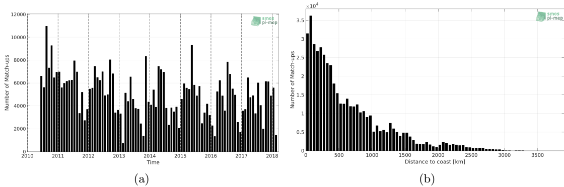
Figure 1: Number of match-ups between TSG-LEGOS-DM and SMOS-L2-DPGS-v662 SSS as a function of time (a) and as function of the distance to coast (b) over the Tropical Pacific Ocean Pi-MEP region and for the full satellite product period.
