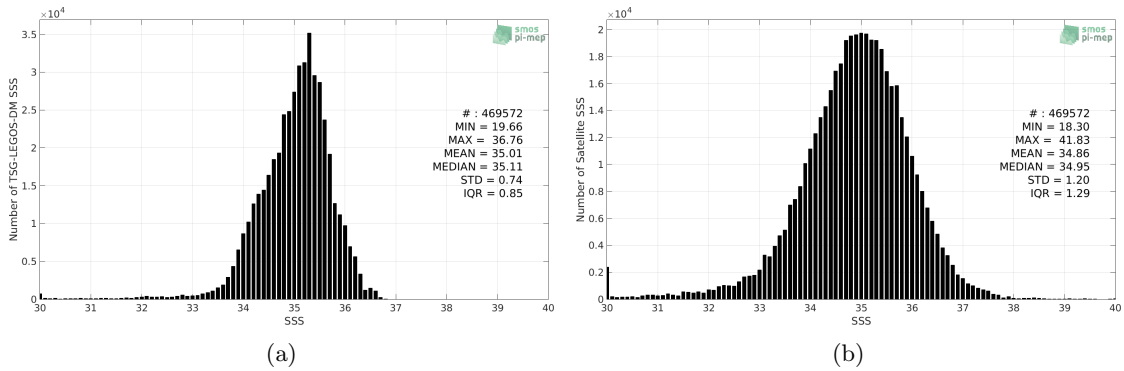
Figure 2: Histograms of SSS from TSG-LEGOS-DM (a) and SMOS-L2-DPGS-v662 (b) considering all match-up pairs per bins of 0.1 over the Tropical Pacific Ocean Pi-MEP region and for the full satellite product period.
