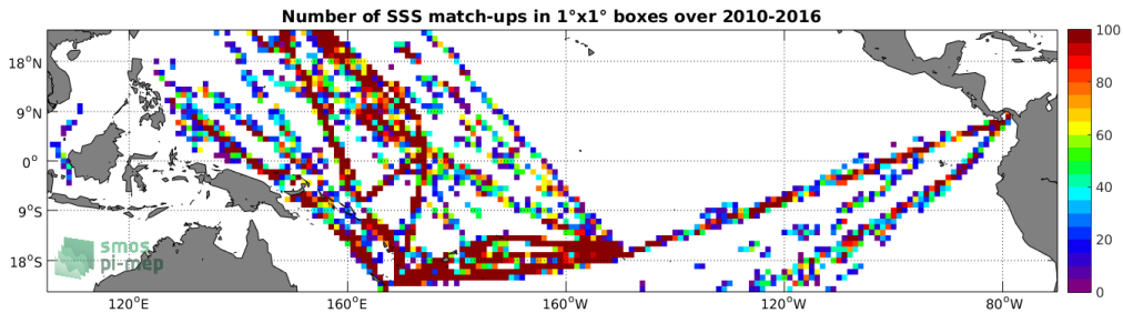
Figure 4: Number of SSS match-ups between TSG-LEGOS-DM SSS and the SMOS-L2-DPGS-v662 SSS product for the Tropical Pacific Ocean Pi-MEP region over 1^\circ \times 1^\circ boxes and for the full satellite product period.
