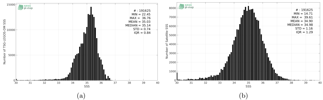
Figure 2: Histograms of SSS from TSG-LEGOS-DM (a) and SMOS-L2-DPGS-v662 (b) considering all match-up pairs per bins of 0.1 over the Tropical Pacific Ocean Pi-MEP region and for the full satellite product period.
