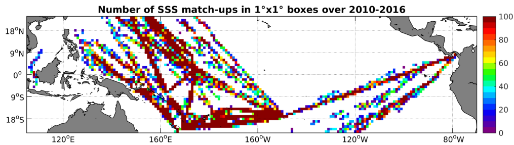
Figure 4: Number of SSS match-ups between TSG-LEGOS-DM SSS and the SMOS-L2-DPGS-v662 SSS product for the Tropical Pacific Ocean Pi-MEP region over 1^\circ \times 1^\circ boxes and for the full satellite product period.
