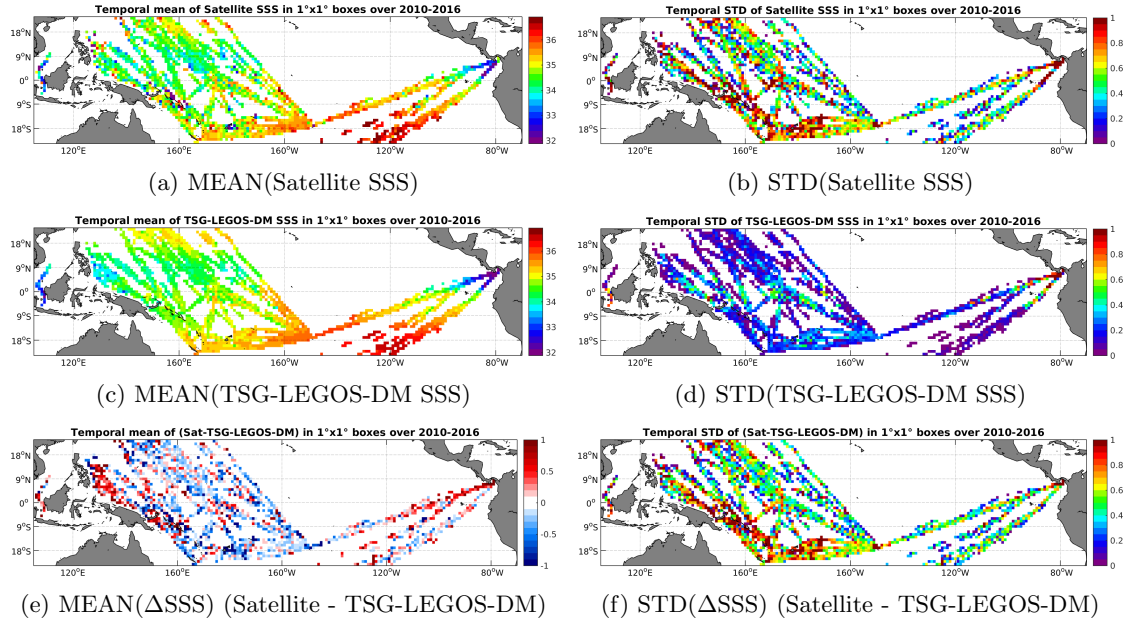
Figure 6: Temporal mean (left) and STD (right) of SSS from SMOS-L2-DPGS-v662 (top), TSG-LEGOS-DM (middle), and of \Delta SSS (Satellite - TSG-LEGOS-DM). Only match-up pairs are used to generate these maps.
