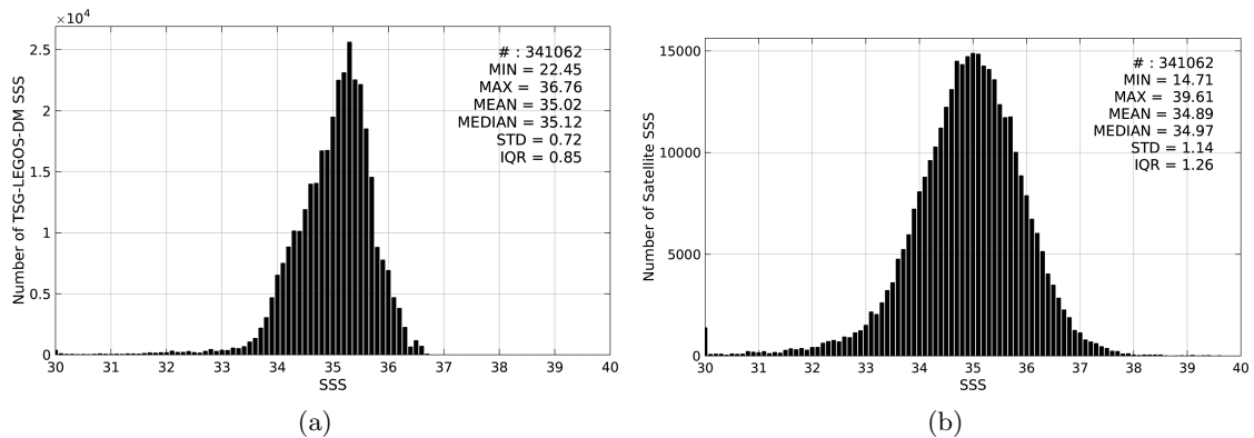
Figure 2: Histograms of SSS from TSG-LEGOS-DM (a) and SMOS-L2-DPGS-v662 (b) considering all match-up pairs per bins of 0.1 over the Tropical Pacific Ocean Pi-MEP region and for the full satellite product period.
