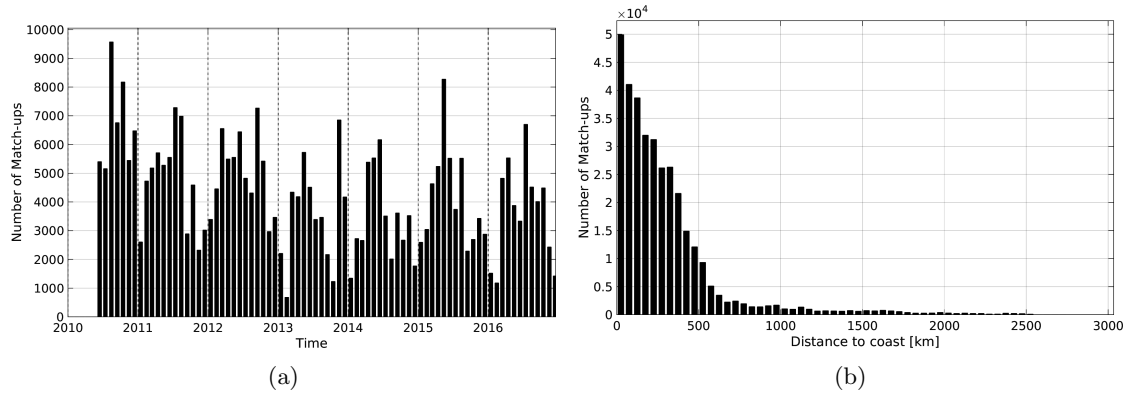
Figure 1: Number of match-ups between TSG-LEGOS-DM and SMOS-L2-DPGS-v662 SSS as a function of time (a) and as function of the distance to coast (b) over the Tropical Pacific Ocean Pi-MEP region and for the full satellite product period.
