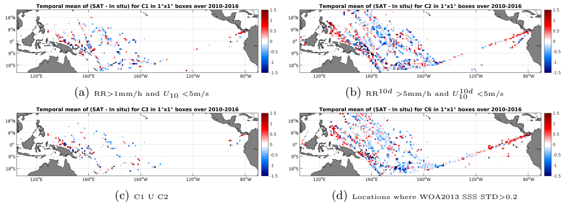
Figure 12: Temporal mean gridded over spatial boxes of size 1^\circ \times 1^\circ of \Delta SSS (SMOS-L2-DPGS-v662 - TSG-LEGOS-DM) for 4 different subdatasets corresponding to: RR > 1\text{mm/h} and U_{10} < 5\text{m/s} (a), RR^{10d} > 5\text{mm/h} and U_{10}^{10d} < 5\text{m/s} (b), C1 U C2 (c), Locations where WOA2013 SSS STD > 0.2 (d).
