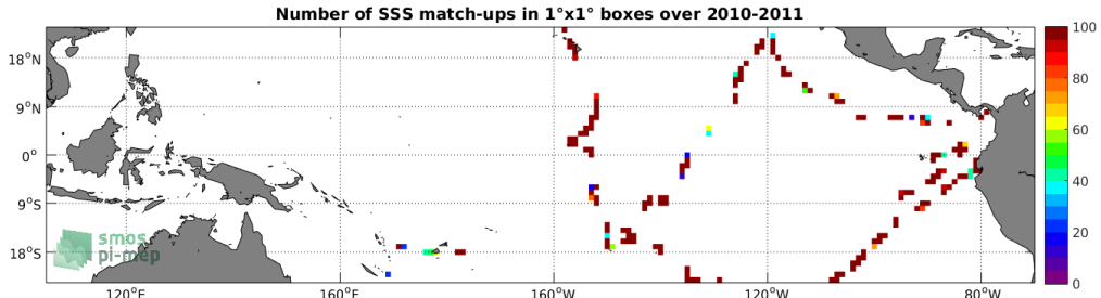
Figure 4: Number of SSS match-ups between TSG (GOSUD-Sailing-ship) SSS and the SMOS SSS L2 v662 (ESA) SSS product for the Tropical Pacific Ocean Pi-MEP region over 1^\circ \times 1^\circ boxes and for the full satellite product period.
