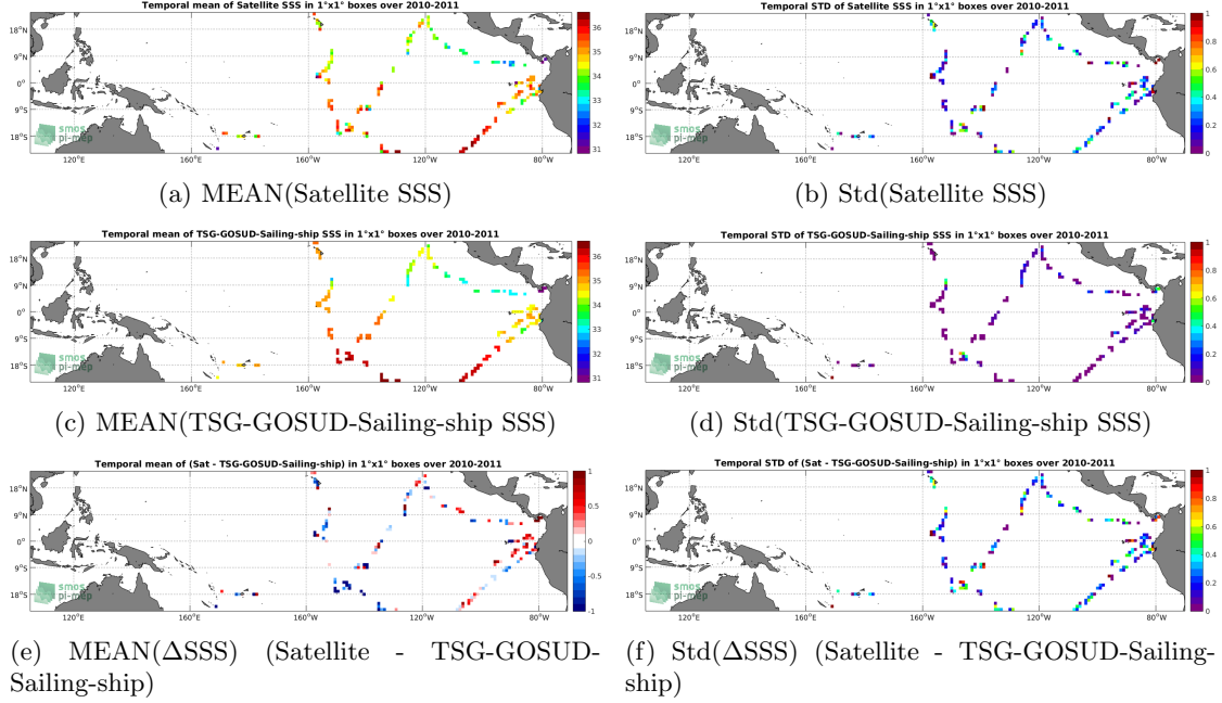
Figure 6: Temporal mean (left) and Std (right) of SSS from SMOS L2 v662 (ESA) (top), TSG-GOSUD-Sailing-ship (middle), and of \Delta SSS (Satellite - TSG-GOSUD-Sailing-ship). Only match-up pairs are used to generate these maps.
