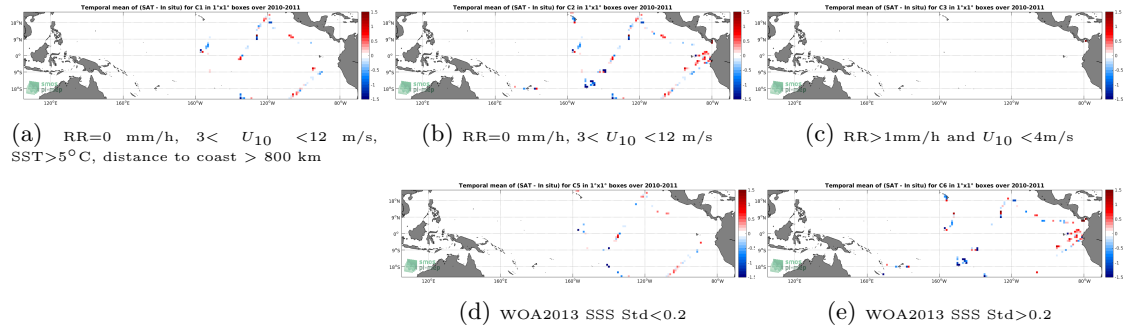
Figure 12: Temporal mean gridded over spatial boxes of size 1^\circ \times 1^\circ of \Delta SSS (SMOS L2 v662 (ESA) - TSG-GOSUD-Sailing-ship) for 5 different subdatasets corresponding to: RR=0 mm/h, 3 < U_{10} < 12 m/s, SST > 5^\circ\text{C} , distance to coast > 800 km (a), RR=0 mm/h, 3 < U_{10} < 12 m/s (b), RR > 1\text{mm/h} and U_{10} < 4\text{m/s} (c), WOA2013 SSS Std < 0.2 (d), WOA2013 SSS Std > 0.2 (e).
