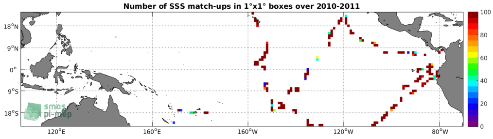
Figure 4: Number of SSS match-ups between TSG-GOSUD-Sailing-ship SSS and the SMOS L2 v662 (ESA) SSS product for the Tropical Pacific Ocean Pi-MEP region over 1^\circ \times 1^\circ boxes and for the full satellite product period.
