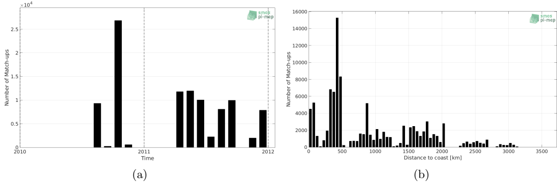
Figure 1: Number of match-ups between TSG-GOSUD-Sailing-ship and SMOS L2 v662 (ESA) SSS as a function of time (a) and as function of the distance to coast (b) over the Tropical Pacific Ocean Pi-MEP region and for the full satellite product period.
