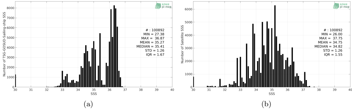
Figure 2: Histograms of SSS from TSG-GOSUD-Sailing-ship (a) and SMOS L2 v662 (ESA) (b) considering all match-up pairs per bins of 0.1 over the Tropical Pacific Ocean Pi-MEP region and for the full satellite product period.
