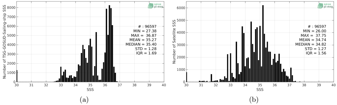
Figure 2: Histograms of SSS from TSG-GOSUD-Sailing-ship (a) and SMOS-L2-DPGS-v662 (b) considering all match-up pairs per bins of 0.1 over the Tropical Pacific Ocean Pi-MEP region and for the full satellite product period.
