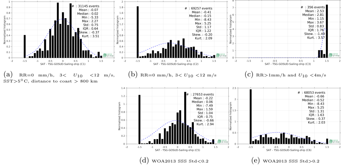
Figure 13: Normalized histogram of \Delta SSS (SMOS-L2-DPGS-v662 - TSG-GOSUD-Sailing-ship) for 5 different subdatasets corresponding to: RR=0 mm/h, 3 < U_{10} < 12 m/s, SST>5°C, distance to coast > 800 km (a), RR=0 mm/h, 3 < U_{10} < 12 m/s (b), RR>1mm/h and U_{10} < 4 m/s (c), WOA2013 SSS Std<0.2 (d), WOA2013 SSS Std>0.2 (e).
