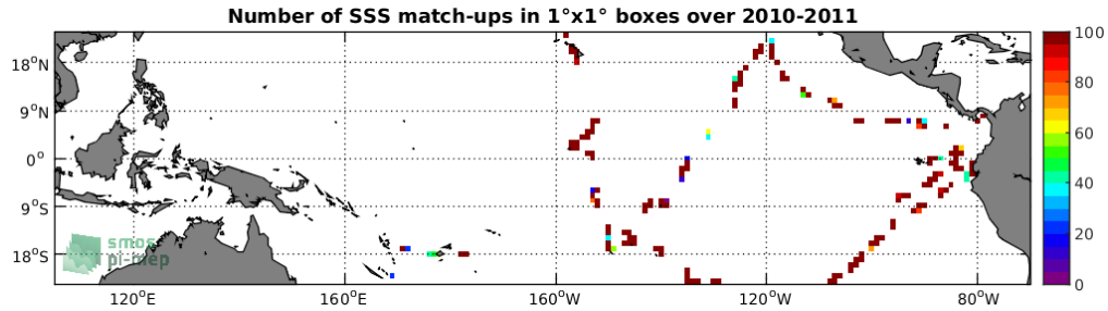
Figure 4: Number of SSS match-ups between TSG-GOSUD-Sailing-ship SSS and the SMOS-L2-DPGS-v662 SSS product for the Tropical Pacific Ocean Pi-MEP region over 1°x1° boxes and for the full satellite product period.
