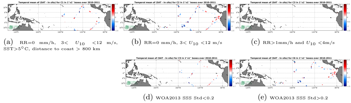
Figure 12: Temporal mean gridded over spatial boxes of size 1^\circ \times 1^\circ of \Delta SSS (SMOS-L2-DPGS-v662 - TSG-GOSUD-Sailing-ship) for 5 different subdatasets corresponding to: RR=0 mm/h, 3 < U_{10} < 12 m/s, SST > 5^\circ C , distance to coast > 800 km (a), RR=0 mm/h, 3 < U_{10} < 12 m/s (b), RR > 1 mm/h and U_{10} < 4 m/s (c), WOA2013 SSS Std < 0.2 (d), WOA2013 SSS Std > 0.2 (e).
