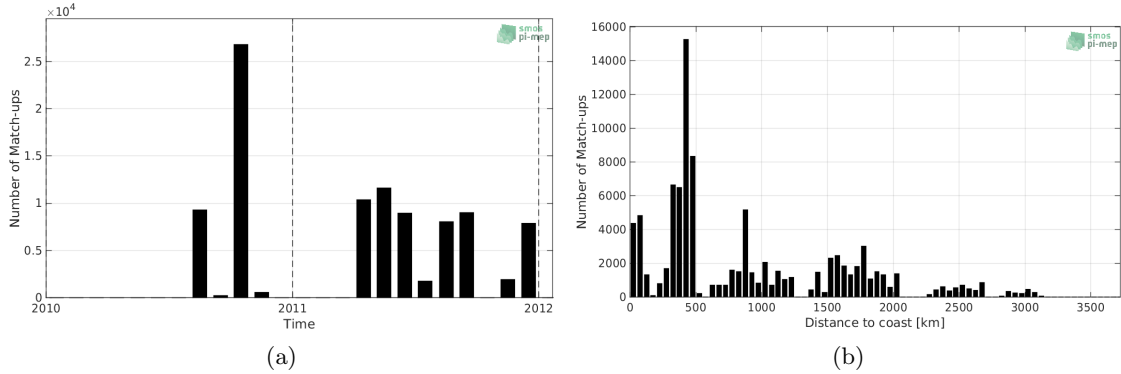
Figure 1: Number of match-ups between TSG-GOSUD-Sailing-ship and SMOS-L2-DPGS-v662 SSS as a function of time (a) and as function of the distance to coast (b) over the Tropical Pacific Ocean Pi-MEP region and for the full satellite product period.
