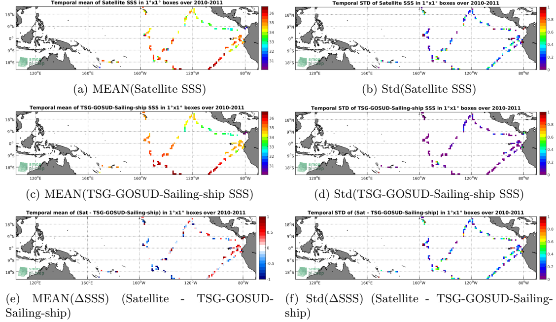
Figure 6: Temporal mean (left) and Std (right) of SSS from SMOS-L2-DPGS-v662 (top), TSG-GOSUD-Sailing-ship (middle), and of \Delta SSS (Satellite - TSG-GOSUD-Sailing-ship). Only match-up pairs are used to generate these maps.
