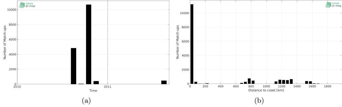
Figure 1: Number of match-ups between TSG-GOSUD-Sailing-ship and SMOS-L2-DPGS-v662 SSS as a function of time (a) and as function of the distance to coast (b) over the Tropical Pacific Ocean Pi-MEP region and for the full satellite product period.
