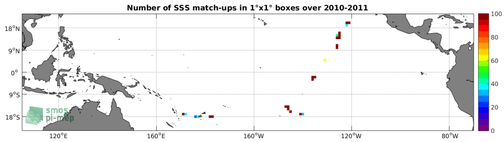
Figure 4: Number of SSS match-ups between TSG-GOSUD-Sailing-ship SSS and the SMOS-L2-DPGS-v662 SSS product for the Tropical Pacific Ocean Pi-MEP region over 1^\circ \times 1^\circ boxes and for the full satellite product period.
