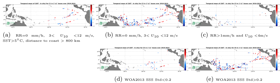
Figure 12: Temporal mean gridded over spatial boxes of size 1^\circ \times 1^\circ of \Delta SSS (SMOS SSS L2 v662 (ESA) - TSG (GOSUD-Research-vessel)) for 5 different subdatasets corresponding to: RR=0 mm/h, 3 < U_{10} < 12 m/s, SST > 5°C, distance to coast > 800 km (a), RR=0 mm/h, 3 < U_{10} < 12 m/s (b), RR > 1mm/h and U_{10} < 4 m/s (c), WOA2013 SSS Std < 0.2 (d), WOA2013 SSS Std > 0.2 (e).
