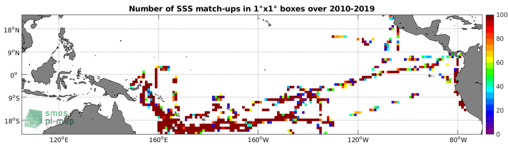
Figure 4: Number of SSS match-ups between TSG (GOSUD-Research-vessel) SSS and the SMOS SSS L2 v662 (ESA) SSS product for the Tropical Pacific Ocean Pi-MEP region over 1^\circ \times 1^\circ boxes and for the full satellite product period.
