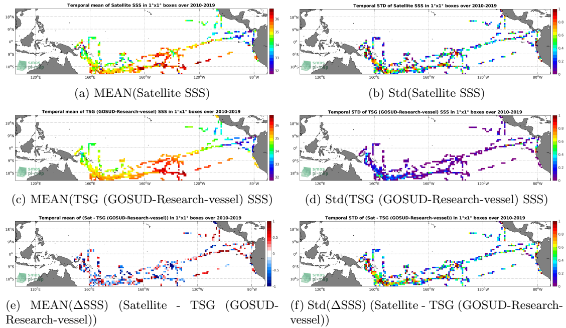
Figure 6: Temporal mean (left) and Std (right) of SSS from SMOS SSS L2 v662 (ESA) (top), TSG (GOSUD-Research-vessel) (middle), and of \Delta SSS (Satellite - TSG (GOSUD-Research-vessel)). Only match-up pairs are used to generate these maps.
