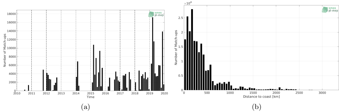
Figure 1: Number of match-ups between TSG (GOSUD-Research-vessel) and SMOS SSS L2 v662 (ESA) SSS as a function of time (a) and as function of the distance to coast (b) over the Tropical Pacific Ocean Pi-MEP region and for the full satellite product period.
