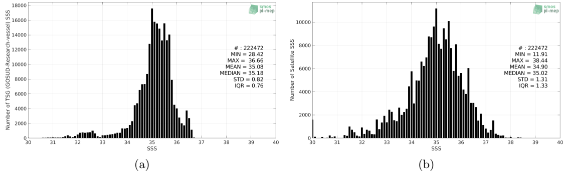
Figure 2: Histograms of SSS from TSG (GOSUD-Research-vessel) (a) and SMOS SSS L2 v662 (ESA) (b) considering all match-up pairs per bins of 0.1 over the Tropical Pacific Ocean Pi-MEP region and for the full satellite product period.
