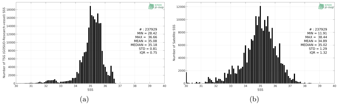
Figure 2: Histograms of SSS from TSG (GOSUD-Research-vessel) (a) and SMOS SSS L2 v662 (ESA) (b) considering all match-up pairs per bins of 0.1 over the Tropical Pacific Ocean Pi-MEP region and for the full satellite product period.
