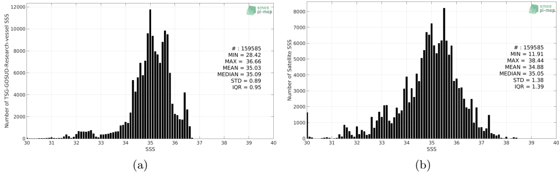
Figure 2: Histograms of SSS from TSG-GOSUD-Research-vessel (a) and SMOS L2 v662 (ESA) (b) considering all match-up pairs per bins of 0.1 over the Tropical Pacific Ocean Pi-MEP region and for the full satellite product period.
