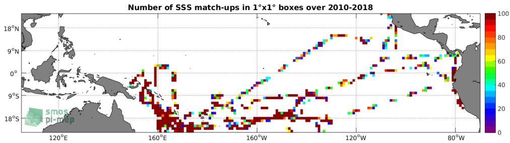
Figure 4: Number of SSS match-ups between TSG-GOSUD-Research-vessel SSS and the SMOS L2 v662 (ESA) SSS product for the Tropical Pacific Ocean Pi-MEP region over 1^\circ \times 1^\circ boxes and for the full satellite product period.
