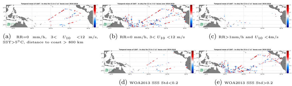
Figure 12: Temporal mean gridded over spatial boxes of size 1^\circ \times 1^\circ of \Delta SSS (SMOS L2 v662 (ESA) - TSG-GOSUD-Research-vessel) for 5 different subdatasets corresponding to:RR=0 mm/h, 3 < U_{10} < 12 m/s, SST > 5^\circ\text{C} , distance to coast > 800 km (a), RR=0 mm/h, 3 < U_{10} < 12 m/s (b), RR > 1 mm/h and U_{10} < 4 m/s (c), WOA2013 SSS Std < 0.2 (d), WOA2013 SSS Std > 0.2 (e).
