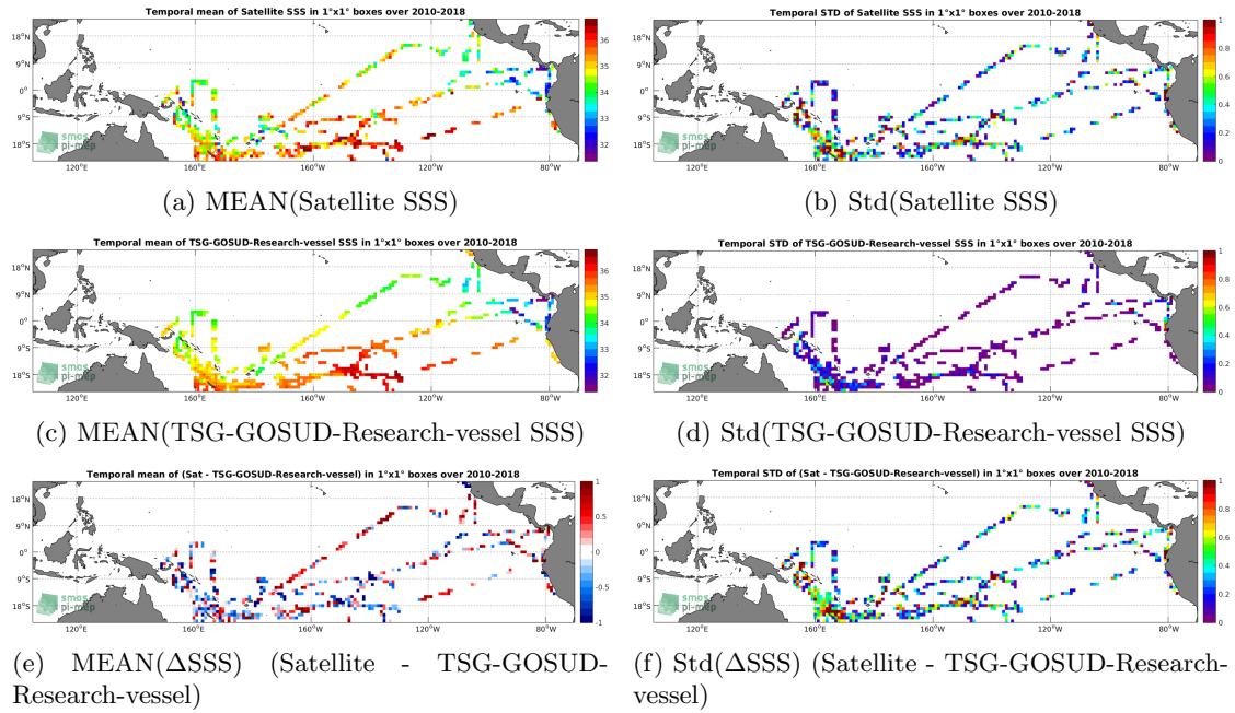
Figure 6: Temporal mean (left) and Std (right) of SSS from SMOS L2 v662 (ESA) (top), TSG-GOSUD-Research-vessel (middle), and of \Delta SSS (Satellite - TSG-GOSUD-Research-vessel). Only match-up pairs are used to generate these maps.
