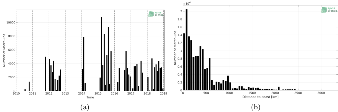
Figure 1: Number of match-ups between TSG-GOSUD-Research-vessel and SMOS L2 v662 (ESA) SSS as a function of time (a) and as function of the distance to coast (b) over the Tropical Pacific Ocean Pi-MEP region and for the full satellite product period.
