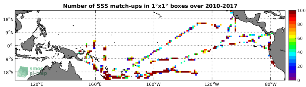
Figure 4: Number of SSS match-ups between TSG-GOSUD-Research-vessel SSS and the SMOS-L2-DPGS-v662 SSS product for the Tropical Pacific Ocean Pi-MEP region over 1^\circ \times 1^\circ boxes and for the full satellite product period.
