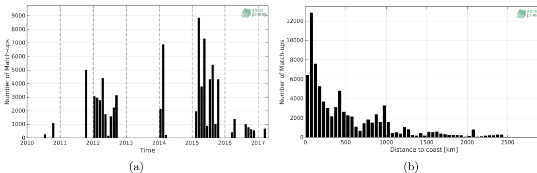
Figure 1: Number of match-ups between TSG-GOSUD-Research-vessel and SMOS-L2-DPGS-v662 SSS as a function of time (a) and as function of the distance to coast (b) over the Tropical Pacific Ocean Pi-MEP region and for the full satellite product period.
