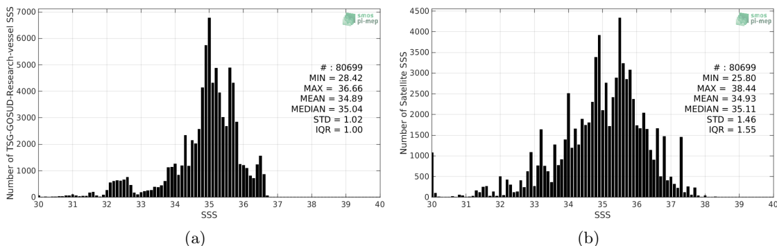
Figure 2: Histograms of SSS from TSG-GOSUD-Research-vessel (a) and SMOS-L2-DPGS-v662 (b) considering all match-up pairs per bins of 0.1 over the Tropical Pacific Ocean Pi-MEP region and for the full satellite product period.
