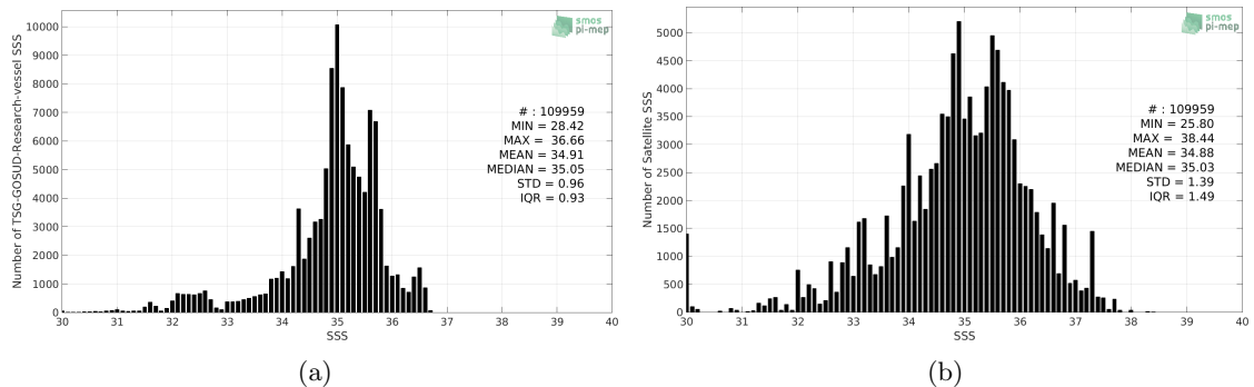
Figure 2: Histograms of SSS from TSG-GOSUD-Research-vessel (a) and SMOS-L2-DPGS-v662 (b) considering all match-up pairs per bins of 0.1 over the Tropical Pacific Ocean Pi-MEP region and for the full satellite product period.
