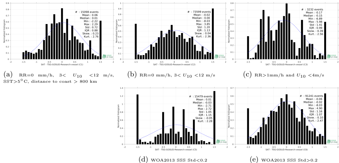
Figure 13: Normalized histogram of \Delta SSS (SMOS-L2-DPGS-v662 - TSG-GOSUD-Research-vessel) for 5 different subdatasets corresponding to: RR=0 mm/h, 3 < U_{10} < 12 m/s, SST >5^\circ C, distance to coast > 800 km (a), RR=0 mm/h, 3 < U_{10} < 12 m/s (b), RR >1 mm/h and U_{10} < 4 m/s (c), WOA2013 SSS Std <0.2 (d), WOA2013 SSS Std >0.2 (e).
